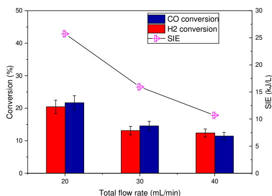
Figure 9. The SIE and conversions as a function of total flow rate (H 2 to CO=1:1, frequency: 3000 Hz, peak-to-peak voltage: 6 kV)
