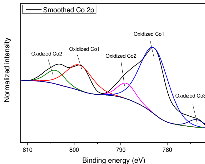
Figure 5. XPS peaking in the Co 2p region of the 20Cl-S sample
