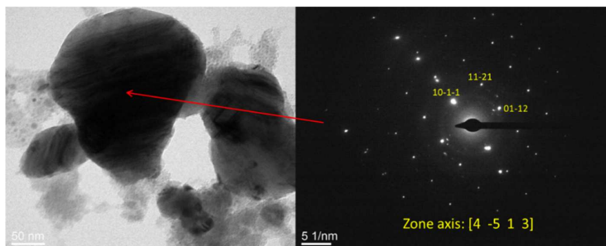
Figure 7. The HRTEM bright field images and selected area diffraction of 20Cl-S sample
