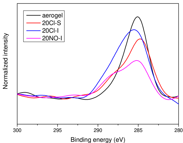
Figure 13. XPS peak region in C1s of the corresponding catalysts after the plasma experiments (smoothed by Gaussian method): Aerogel, 20Cl-S, 20Cl-I, 20NO-I
