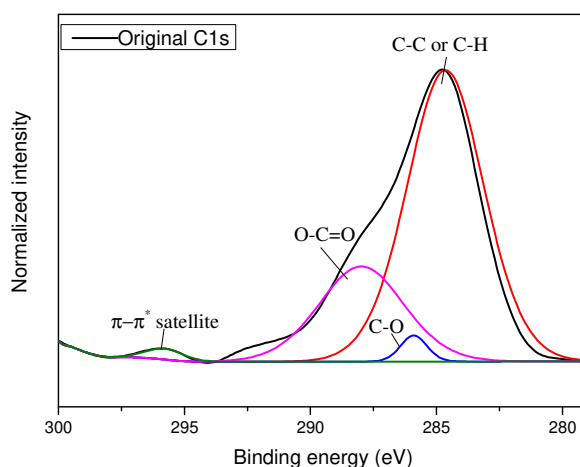
Figure 14. XPS peaking region in C1s of the 20CoCl-sol sample after the plasma experiments
