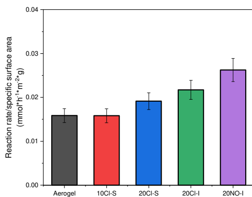
Figure 12. The reaction rates normalized to specific surface area varying by the different catalysts (total flow rate: 30 mL n /min, frequency: 3000 Hz, peak-to-peak voltage: 6 kV)
