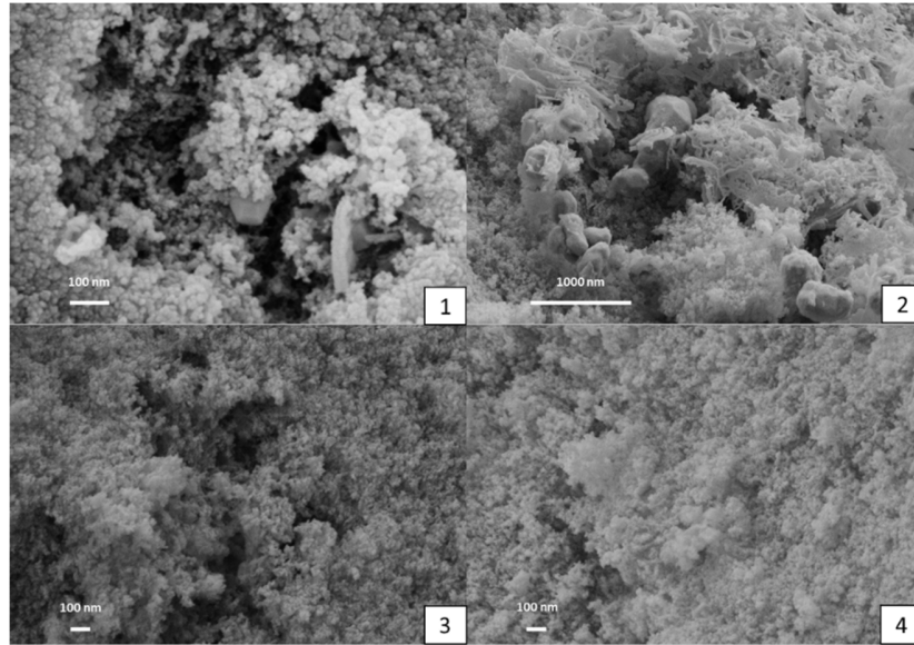
Figure 6. The SEM micrographs of: (1) 10Cl-S, (2) 20Cl-S, (3) 20Cl-I, (4) 20NO-I
