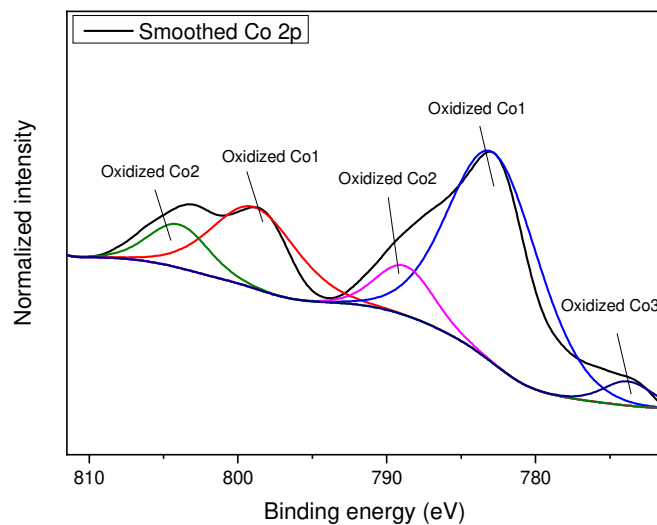
Figure 5. XPS peaking in the Co 2p region of the 20Cl-S sample
