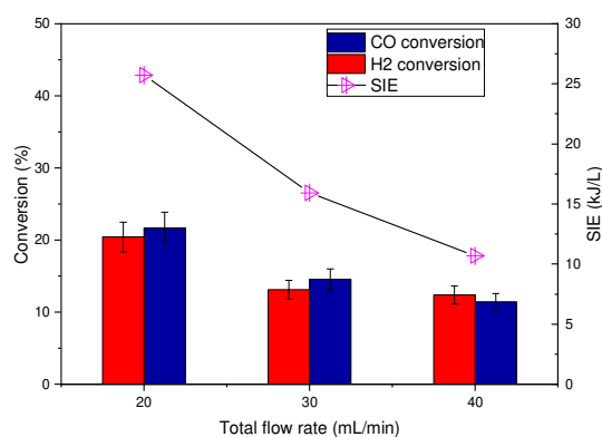
Figure 9. The SIE and conversions as a function of total flow rate (H 2 to CO=1:1, frequency: 3000 Hz, peak-to-peak voltage: 6 kV)
