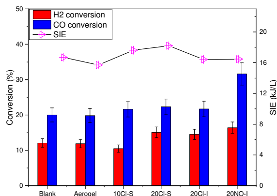
Figure 11. The SIE and conversions varying by the different catalysts (total flow rate: 30 mL n /min, frequency: 3000 Hz, peak-to-peak voltage: 6 kV)
