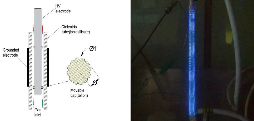
Figure 2. Photo and schematic diagram of the DBD reactor
