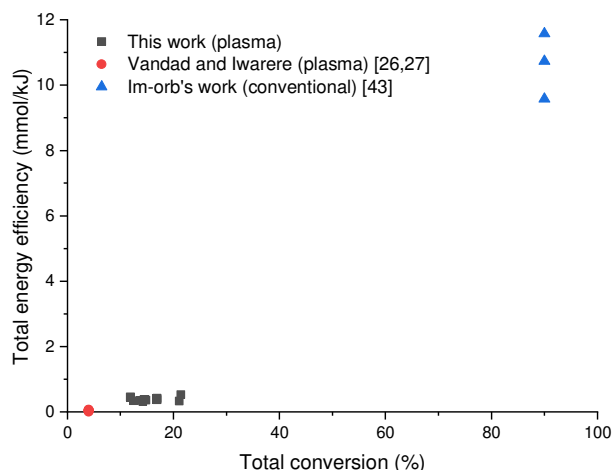
Figure 15. Experimental data collected from the literature for plasma and conventional FTS process, showing total energy efficiency as a function of conversion of reactants.
