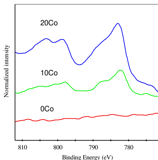
Figure 4. The Co 2p XPS spectra of aerogel, 10Cl-S, and 20 Cl-S samples.
