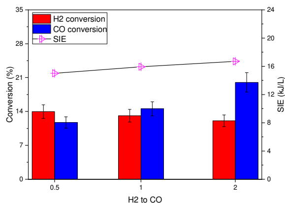
Figure 10. The SIE and conversions as a function of different H 2 to CO ratio (total flow rate: 30 mL n /min, frequency: 3000 Hz, peak-to-peak voltage: 6 kV)
