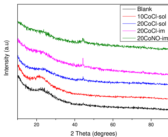
Figure 3. The XRD patterns of the Co/SiO 2 aerogel samples
