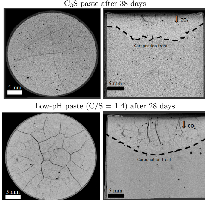
Figure 2: \mu CT scan of samples subjected to accelerated carbonation (voxel size = 17 \mu\text{m} ). Left panel: top view of the sample, right panel: transverse view of the sample. These scans show the evolution of the carbonation front as well as the appearance of cracks. Measurement of the extent of the carbonation front were coupled with XRD profiles, thermogravimetric analysis and phenolphthaleine tests.
