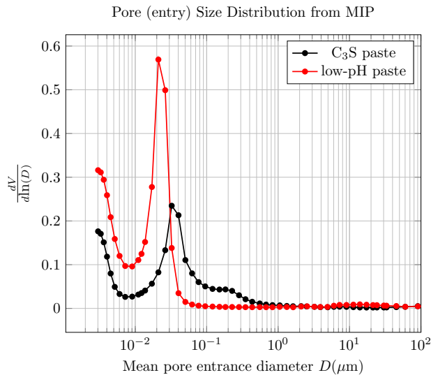
Figure 1: Representation of the pore size distributions of the two samples obtained by MIP, indicating a finer porosity for the low-pH paste.
