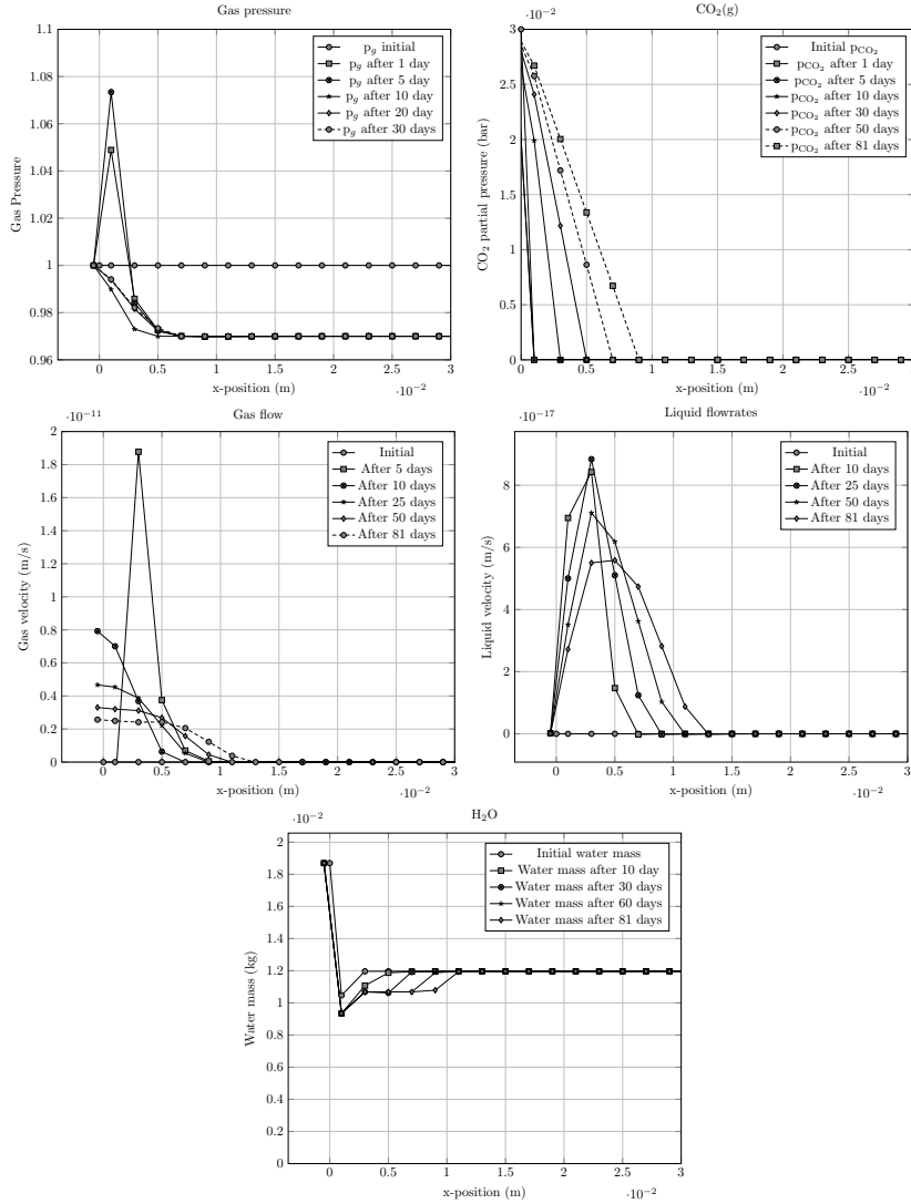
Figure 5: Evolution of gas and liquid flow parameters during the accelerated carbonation.
