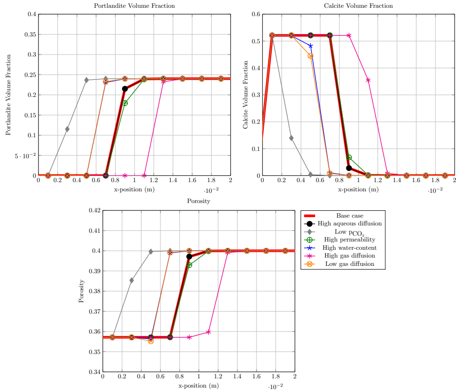
Figure 6: Sensitivity analysis. Comparison between the portlandite, calcite and porosity profiles after 60 days
