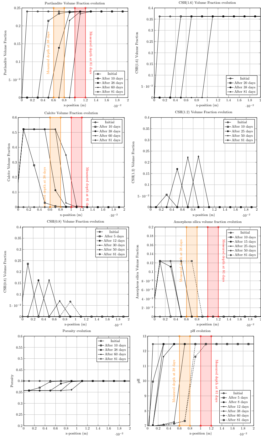
Figure 3: Evolution of the mineral, porosity and pH profiles during accelerated carbonation of the C_3S sample. Highlighted carbonated regions in orange and red correspond to the experimental measurements of the carbonation depths summed up in table 2
