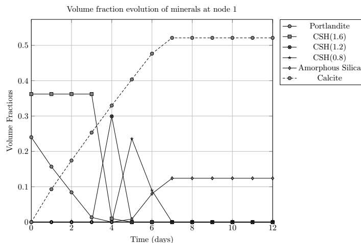
Figure 4: Evolution of mineralogy in the first two millimeters of the \text{C}_3\text{S} paste over time
