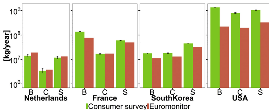
Fig. 3. Total product use estimates [kg/year] for the four countries considered (green bar) compared to estimates from the total market approaches Euromonitor (red bar). B: Bodywash, C: Conditioner, S: Shampoo. The error bars represent the 95% confidence interval of the Monte Carlo results. The results are presented on a logarithmic scale. (For interpretation of the references to colour in this figure legend, the reader is referred to the web version of this article.)
