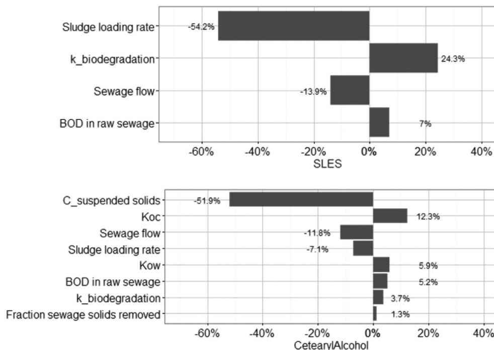
Fig. 5. Relative correlation of the uncertain parameters (with an absolute relative contribution > 1%) used to derive the removal efficiencies of sodium lauryl ether sulfate (SLES, top) and cetearyl alcohol (bottom) from wastewater coupling the SimpleTreat model to a Monte Carlo analysis.
