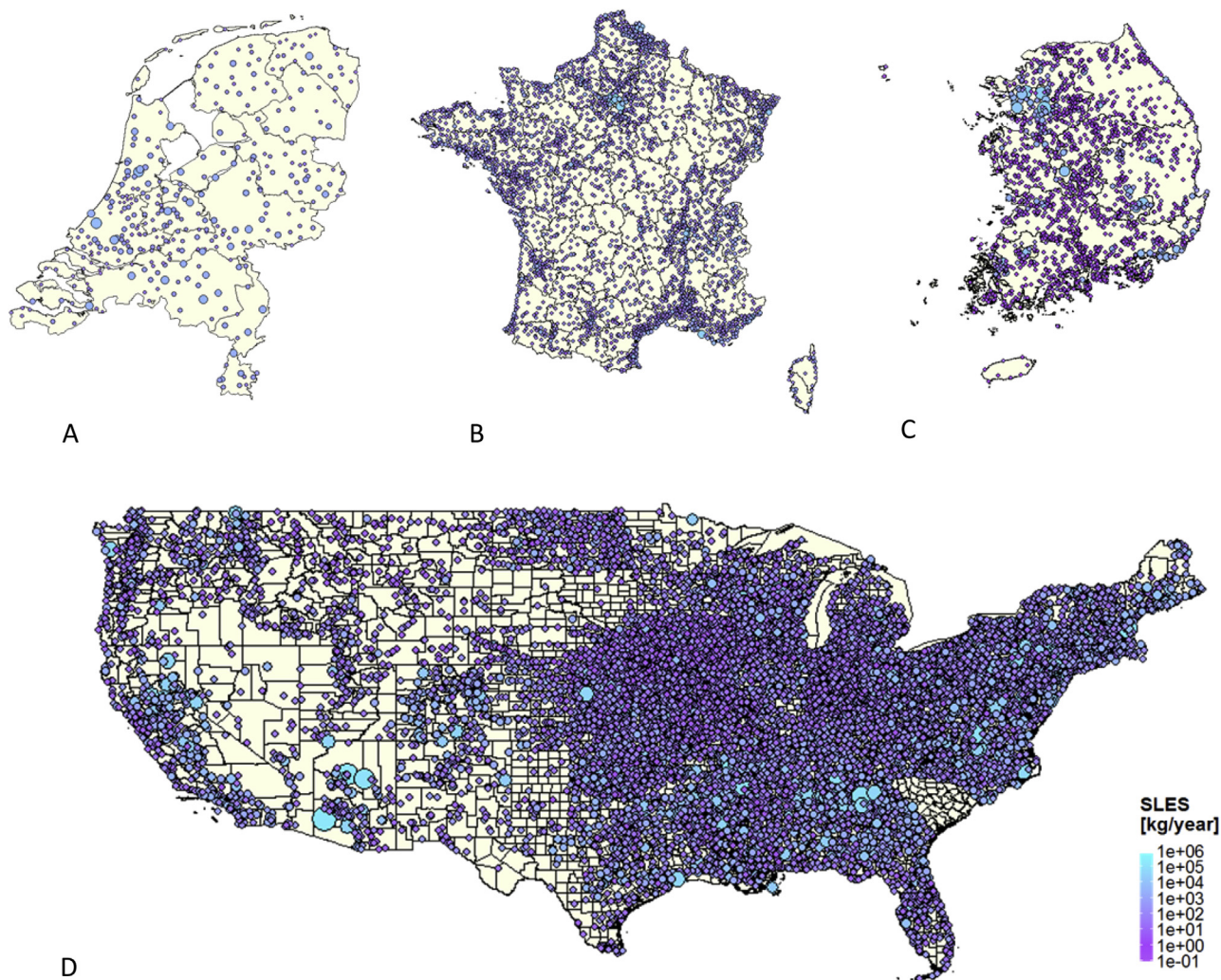
Fig. 2. Geometric mean effluent emission estimates of sodium lauryl ether sulfate (SLES) in the Netherlands (A), France (B), South Korea (C), and the USA (D) resulting from the use of conditioner, bodywash, and shampoo. The size and the color of the dots represent the geometric mean of the emission loads at each WWTP. (For interpretation of the references to colour in this figure legend, the reader is referred to the web version of this article.)
