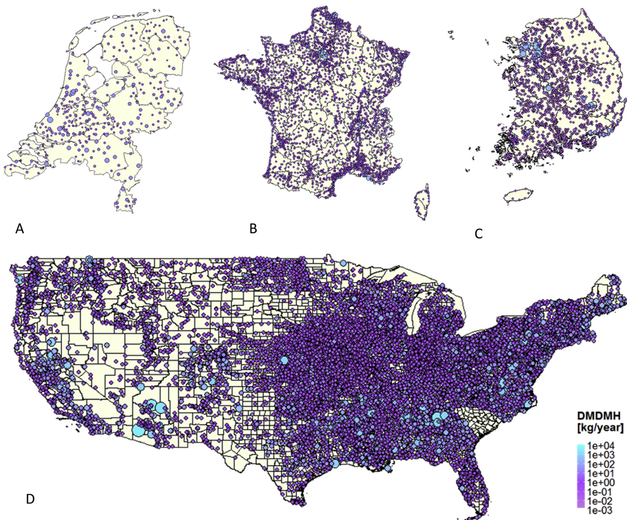
Fig. 1. Geometric mean effluent emission estimates of dimethyloldimethyl hydantoin (DMDMH) in the Netherlands (A), France (B), South Korea (C), and the USA (D) resulting from the use of conditioner, bodywash, and shampoo. The size and the color of the dots represent the geometric mean of the emission loads at each WWTP. (For interpretation of the references to colour in this figure legend, the reader is referred to the web version of this article.)
