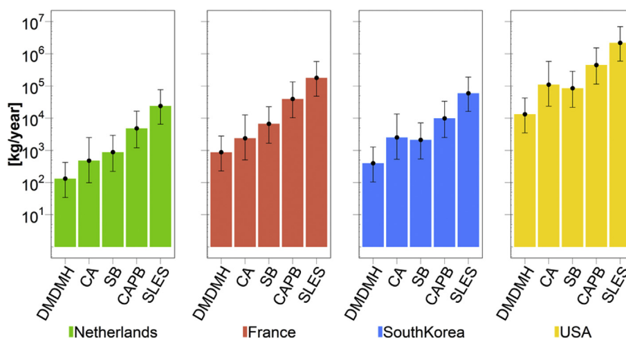
Fig. 4. Chemical emissions in the effluents of WWTPs resulting from the use of shampoo, bodywash and conditioner in the four analysed countries. SLES: sodium lauryl ether sulfate, CAPB: cocamidopropyl betaine, CA: cetearyl alcohol, SB: sodium benzoate, DMDMH: dimethyloldimethyl hydantoin. The error bars represent the 95% confidence interval of the Monte Carlo results.
