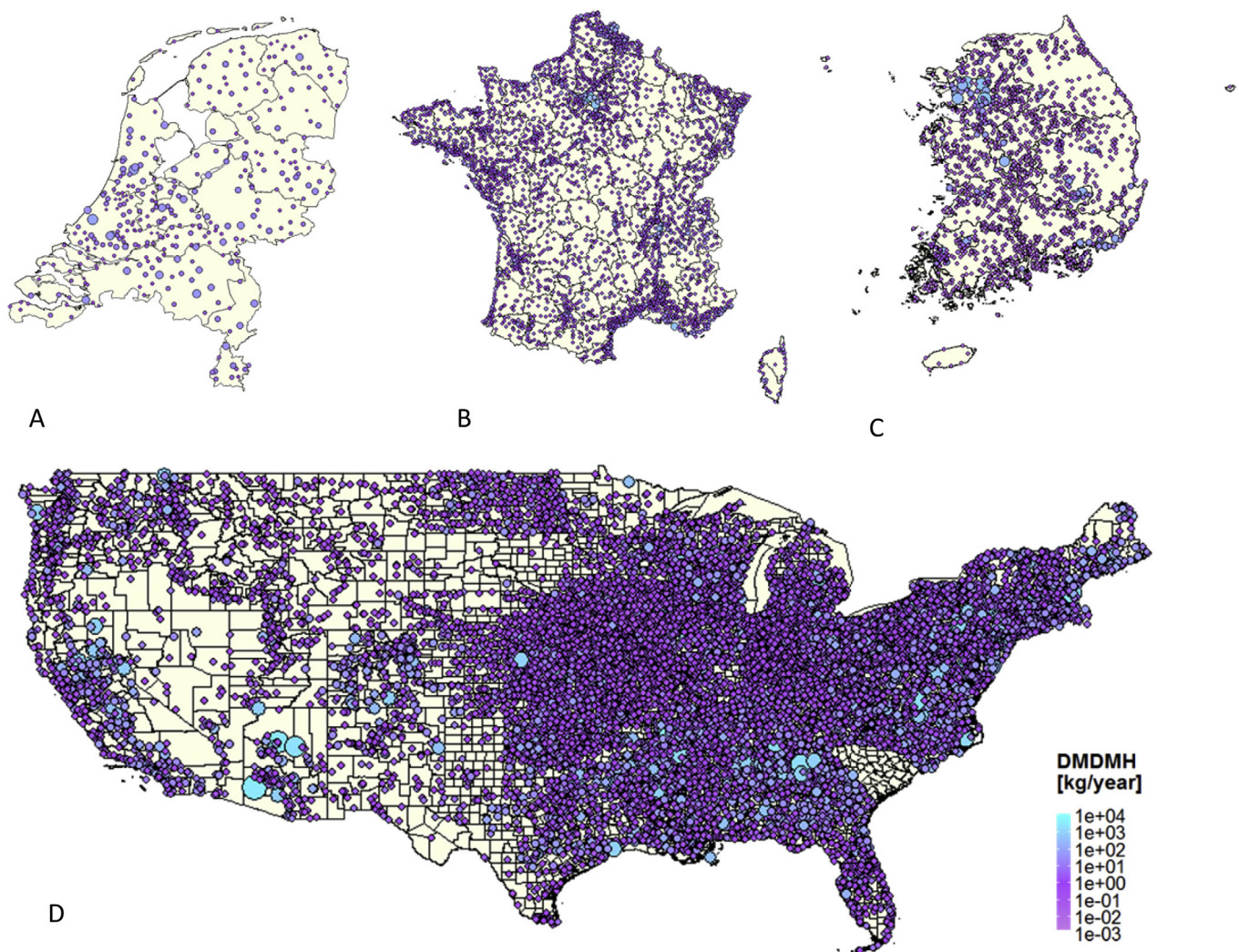
Fig. 1. Geometric mean effluent emission estimates of dimethyloldimethyl hydantoin (DMDMH) in the Netherlands (A), France (B), South Korea (C), and the USA (D) resulting from the use of conditioner, bodywash, and shampoo. The size and the color of the dots represent the geometric mean of the emission loads at each WWTP. (For interpretation of the references to colour in this figure legend, the reader is referred to the web version of this article.)
