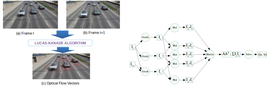
Fig. 2: Workflow of Lucas-Kanade
