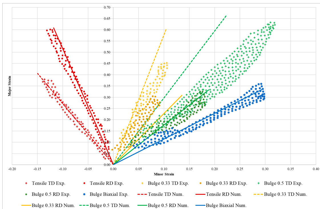
Figure 6. Experimental and numerical strain paths on the major and minor strains diagram from results of the tensile and bulge tests.
