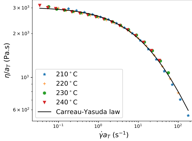
Figure 10: \eta(\dot{\gamma}, T)/\alpha_T vs. \dot{\gamma}\alpha_T for the ABS polymer at four temperatures and solution obtained from the Carreau-Yasuda's law.
