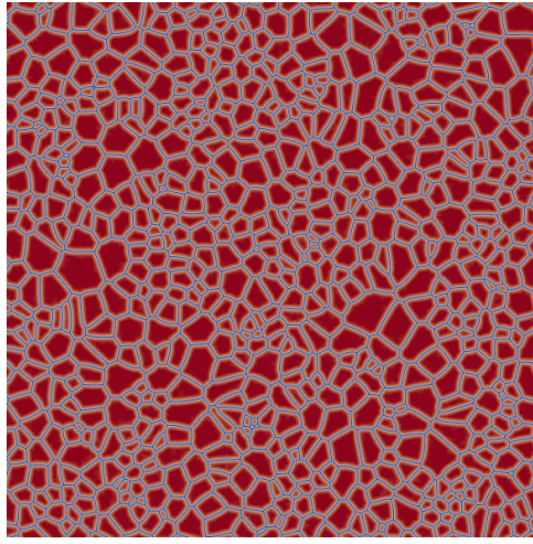
FIGURE 3 – Initial state of the microstructure composed of 1000 grains and built thanks to a Laguerre-Voronoi algorithm.
