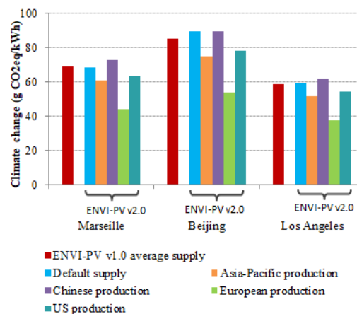
b) Environmental performance of laminated mono-Si PV systems for human toxicity (cancer effects)
