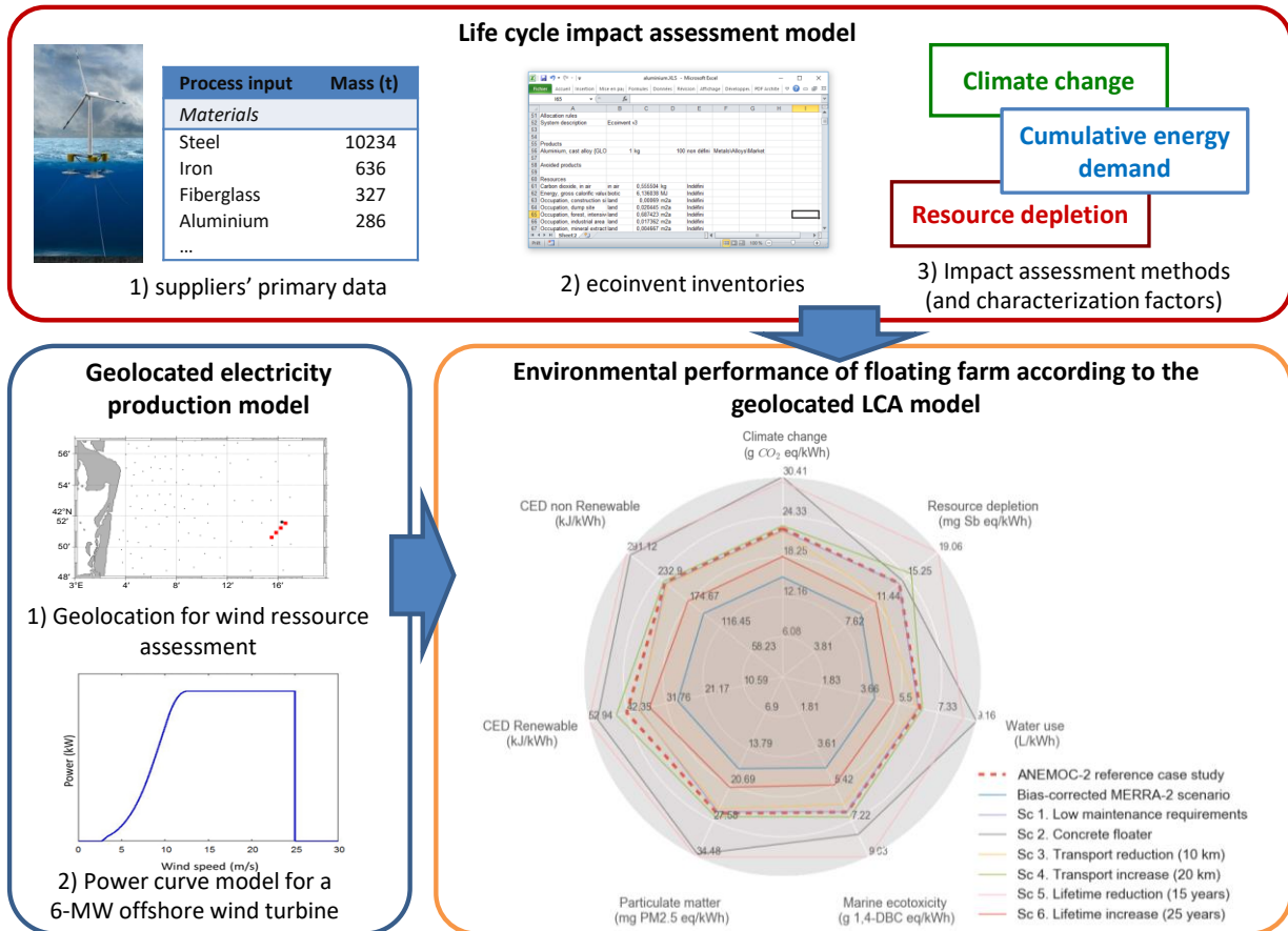
Figure 1: Components of the geolocated LCA model and environmental performance results for the baseline scenario based on ANEMOC-2 database and alternative scenarios evaluated in the sensitivity analysis
