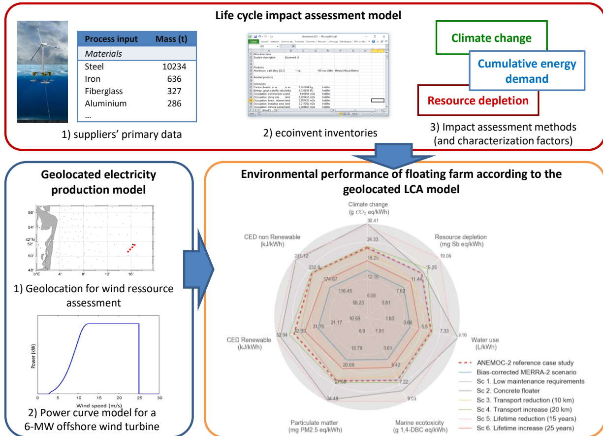
Figure 1: Components of the geolocated LCA model and environmental performance results for the baseline scenario based on ANEMOC-2 database and alternative scenarios evaluated in the sensitivity analysis
