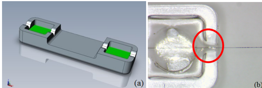
Figure 4. (a) Plastic tabs used for mounting one end of a fibre. (b) Well defined gauge length with proper alignment.
