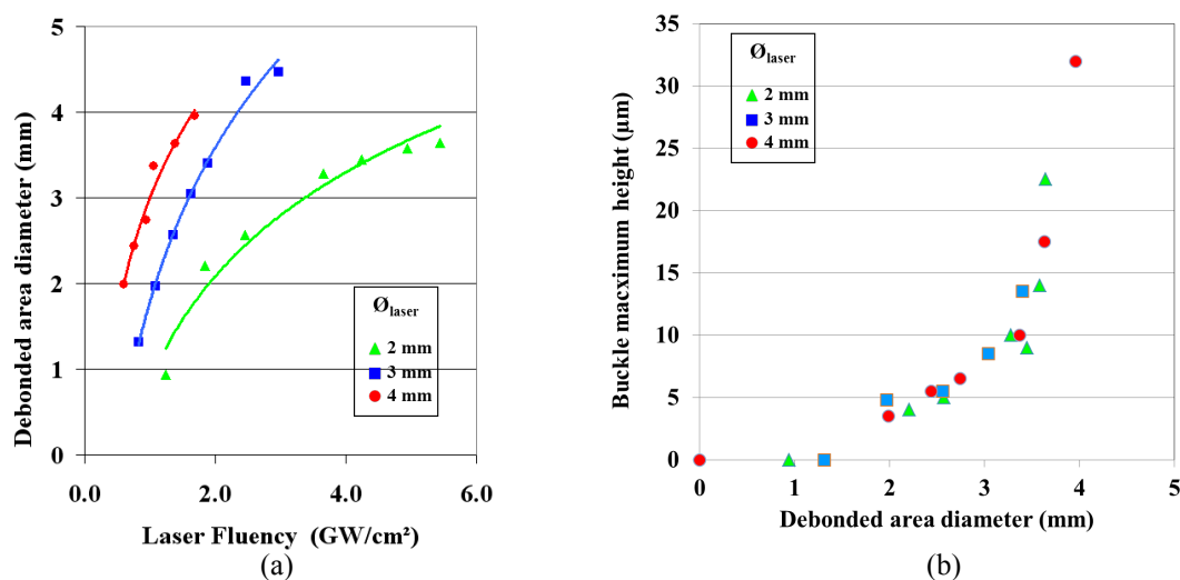
Figure 6: LASAT applied to reference process condition on a rectangular sample (a) LASAT-2D curves for 2mm (green triangle), 3mm (blue square) and 4mm (red dot) of laser shock diameter and (b) evolution of blister height with the size of debonded area (same marker code)
