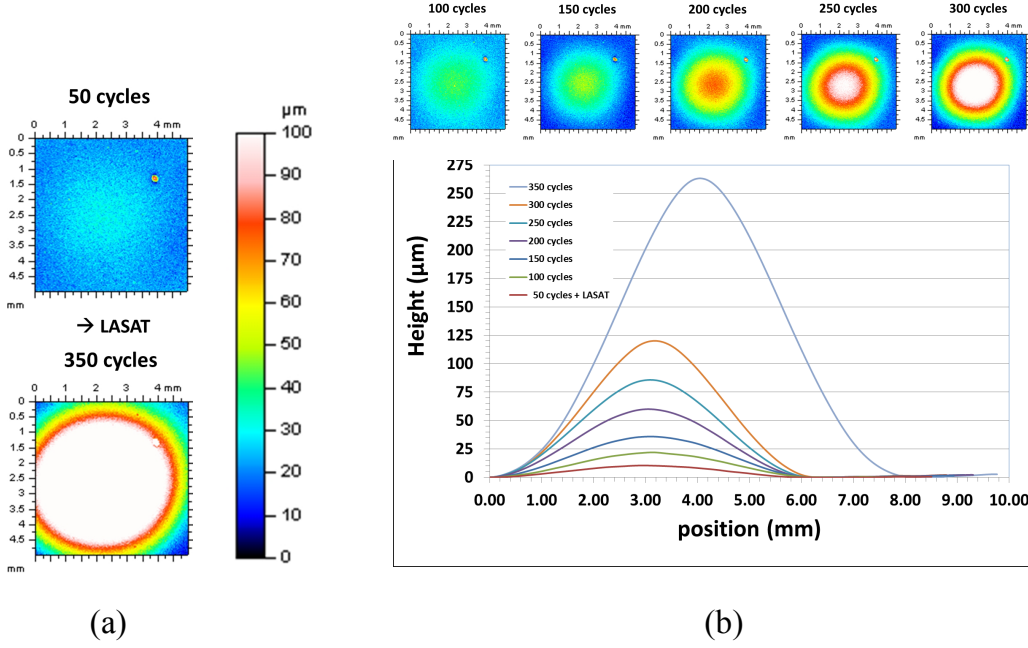
Figure 7: Evolution of blister profile with thermal cycling, initial debonding has been introduced by LASAT after 50 cycles (a) Detail of 3D profilometer measurement at 50 cycles and after 350 cycles (b) Evolution with number of cycles of one profile; inserts amplitude corresponds to (a)
