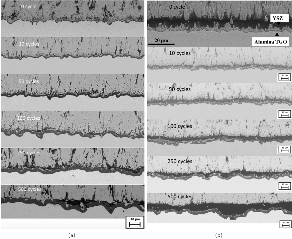
Figure 5: SEM-BSE observation of cross-section for as-processed to 500 thermal cycles at 1100 °C/1h (a) away from the laser shock location (b) through the blister induced by laser shock
