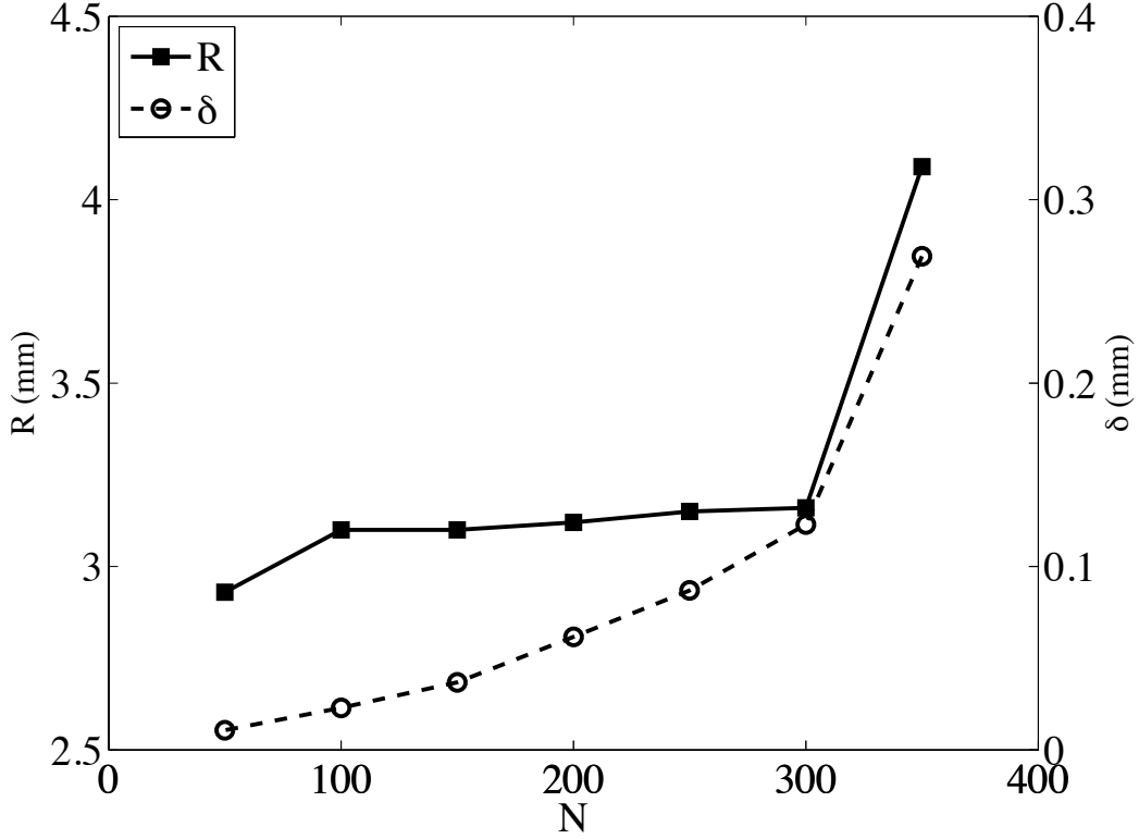
Figure 8: Geometrical evolution of one blister under thermal cycling; an initial delamination has been introduced after 50 cycles, the measurements are the radius R of the blister and its height \delta
