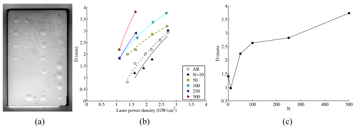
Figure 4: LASAT applied to reference process condition on a rectangular sample (a) surface observation after 500 cycles and (b) LASAT-2D curves for as-processed to 500 thermal cycles at 1100 \text{ }^\circ\text{C}/1\text{h} (c) evolution of debonded diameter as a function of the number of thermal cycles for a laser power density of 1.6 \text{ GW/cm}^2 .
