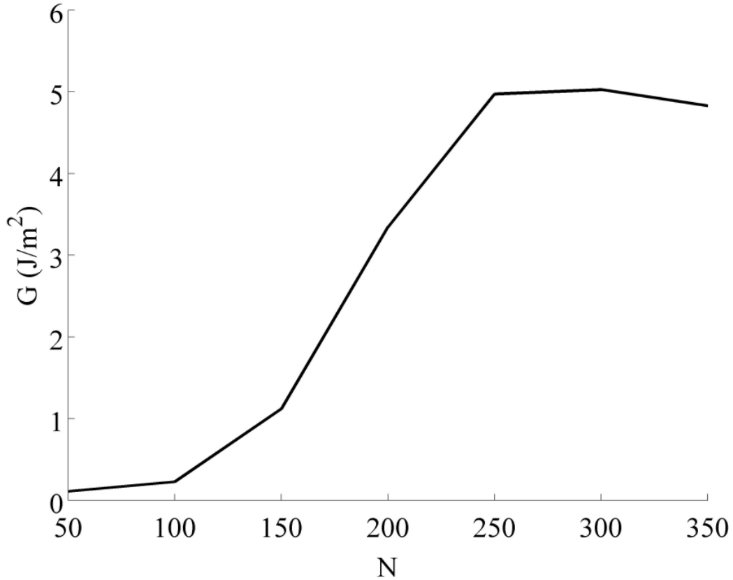
Figure 11: Evolution of energy release rate G as a function of the number of thermal cycles N ; G is derived from pseudo SIF values associated to local measurement of blistering in the vicinity of the crack tip
