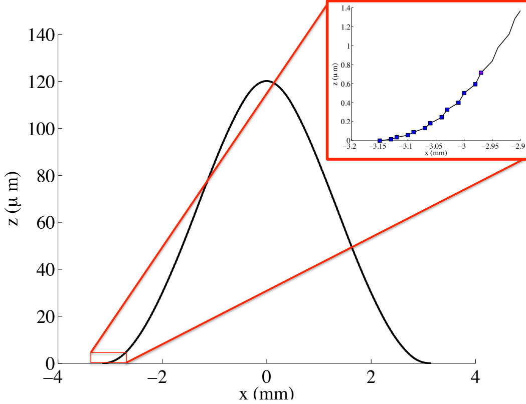
Figure 10: Out-of-plane positions obtained from 3D measurement of the blister for N=300 cycles from Figure 7; insert is magnification of the curve where \delta_y^i is measured see text for details
