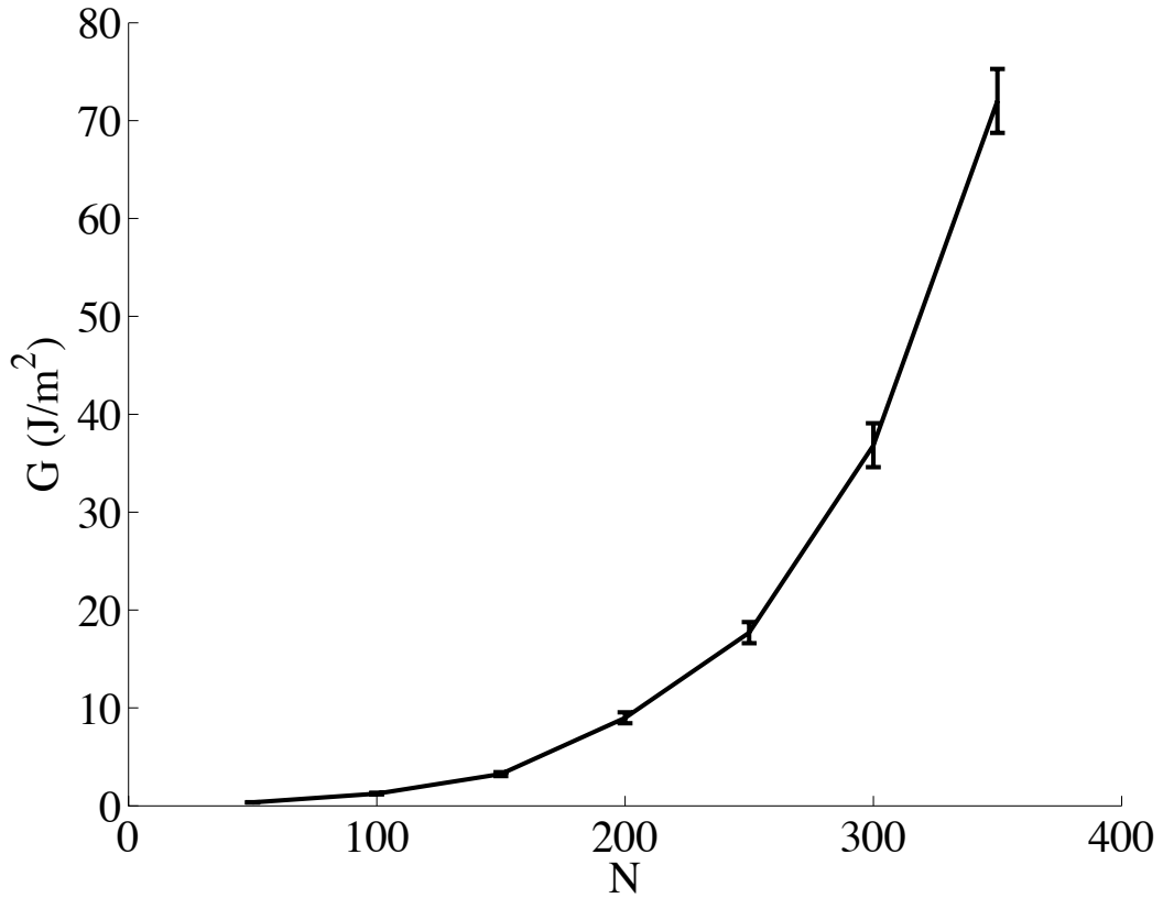
Figure 9: Evolution of energy release rate G as a function of the number of thermal cycles N assuming a blister perfectly clamped on its edge
