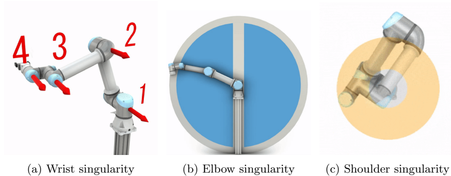
Fig. 3: Singularities of UR robots (source: www.universal-robots.com )
