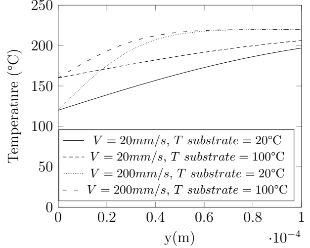
Figure 12: Temperature profile between the printing head and the substrate at the printing head outlet for two printing head velocities 20 and 200 mm/s and two interfacial temperatures 120°C and 160°C corresponding respectively to 20 and 100°C substrate temperatures.
