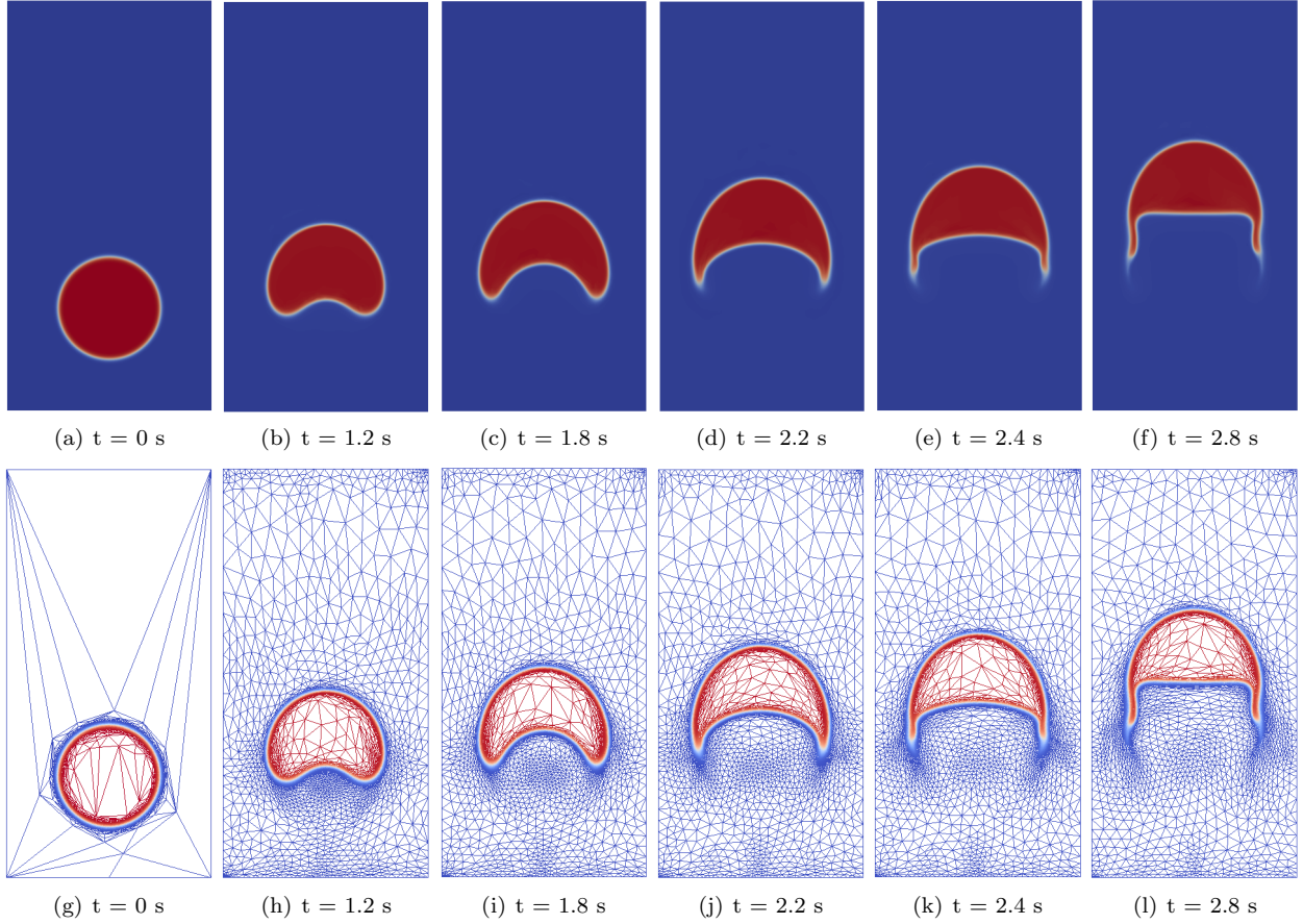
Figure 12: 2D rising bubble evolution and refined meshes
