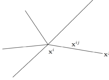
Figure 1: Patch associated with node x^i
