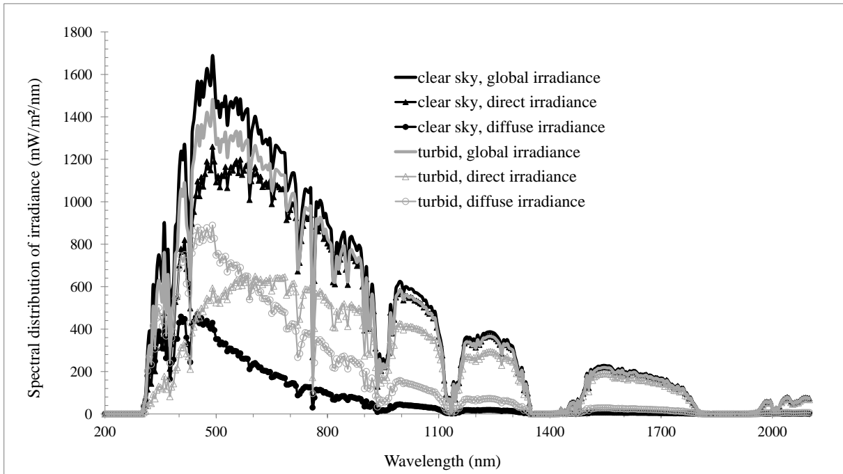
Figure 6.10. Global, direct and diffuse irradiances at ground as a function of wavelength for a solar zenithal angle of 30^\circ and two cases of cloud-free conditions: clear sky (visibility of 50 km) and turbid (visibility of 10 km).
