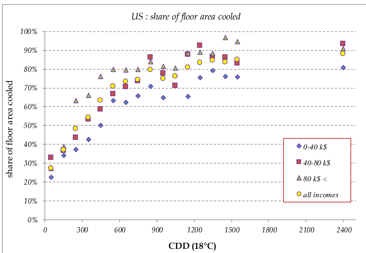
Figure 3: share of floor area cooled, for USA
