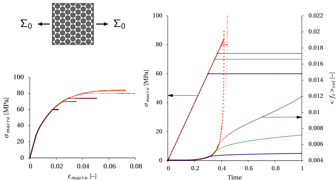
Figure 6 – Durability - Numerical creep tests on an hexagonal pattern cell
