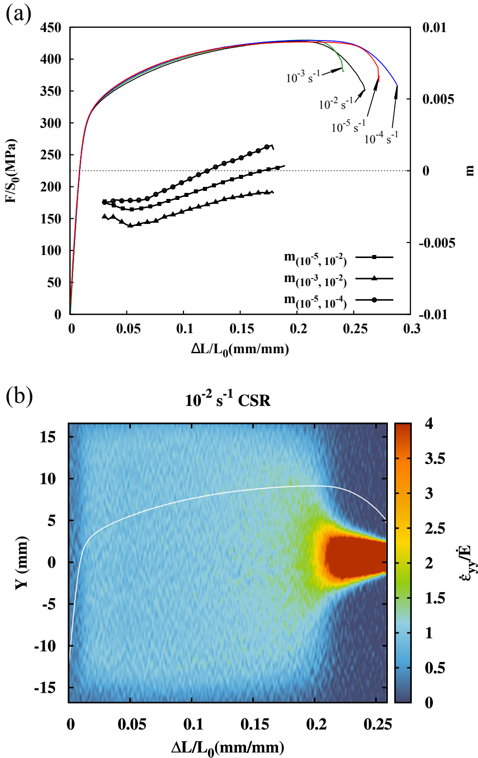
Figure 2: (a) Stress strain curves for constant strain rate (CSR) tests at different strain rates and the strain rate sensitivity evolution calculated from different strain rate pairs. (b) Experimental spatio-temporal pattern of the CSR test at a strain rate 10^{-2} \text{ s}^{-1} ( \Delta t=0.2 \text{ s} ).
