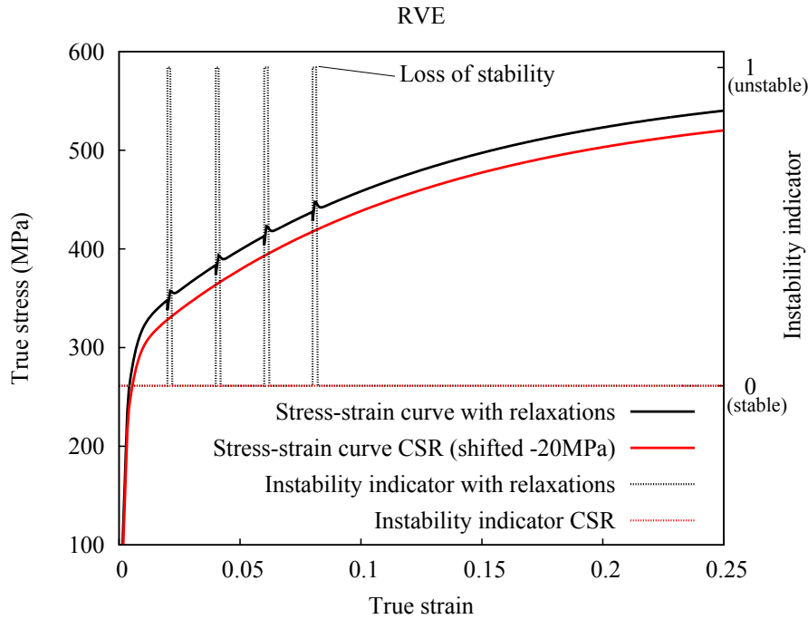
Figure 11: Numerical instability analysis based on a volume element (RVE) performed for both of CSR and relaxation conditions ( \dot{E} = 10^{-2} \text{ s}^{-1} ).
