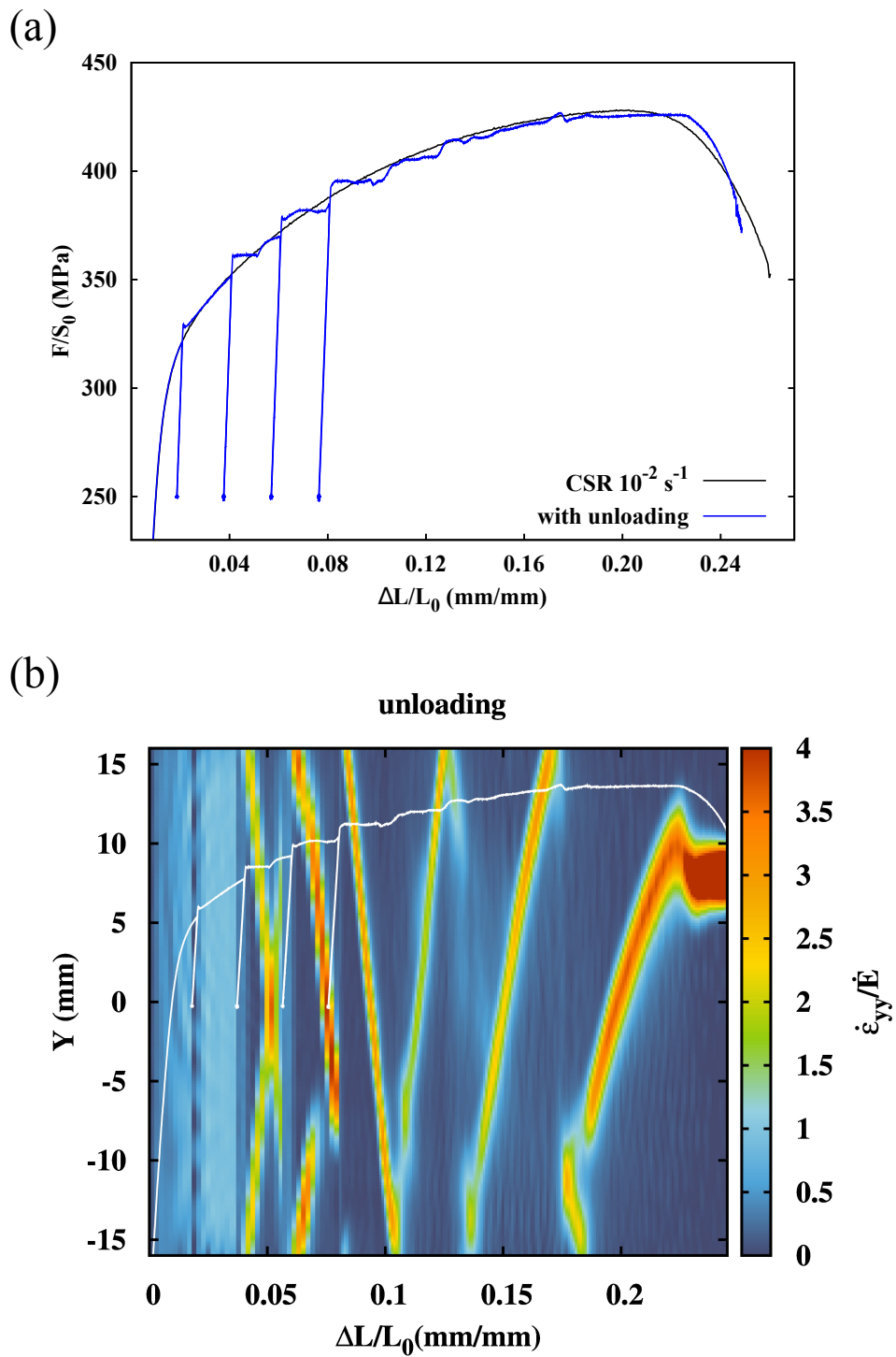
Figure 4: (a) Constant strain rate tensile test at a strain rate 10^{-2} \text{ s}^{-1} (black line) superposed with the curve of tensile test with unloading ageing (blue curve). (b) The experimental spatio-temporal pattern of the tensile test with unloading ageing at a strain rate 10^{-2} \text{ s}^{-1} ( \Delta t = 0.2 \text{ s} ).
