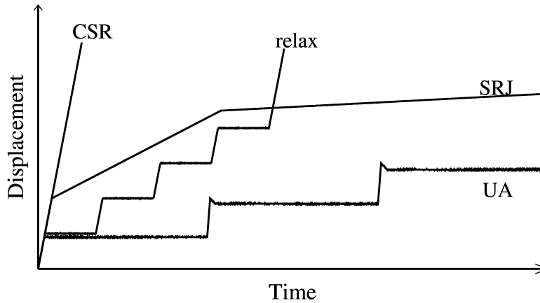
Figure 1: Illustration of displacement evolutions of complex loading tests carried out in this work as function of time: constant strain rate test (CSR), relaxation test (relax), unloading ageing test (UA) and strain rate jump test (SRJ).
