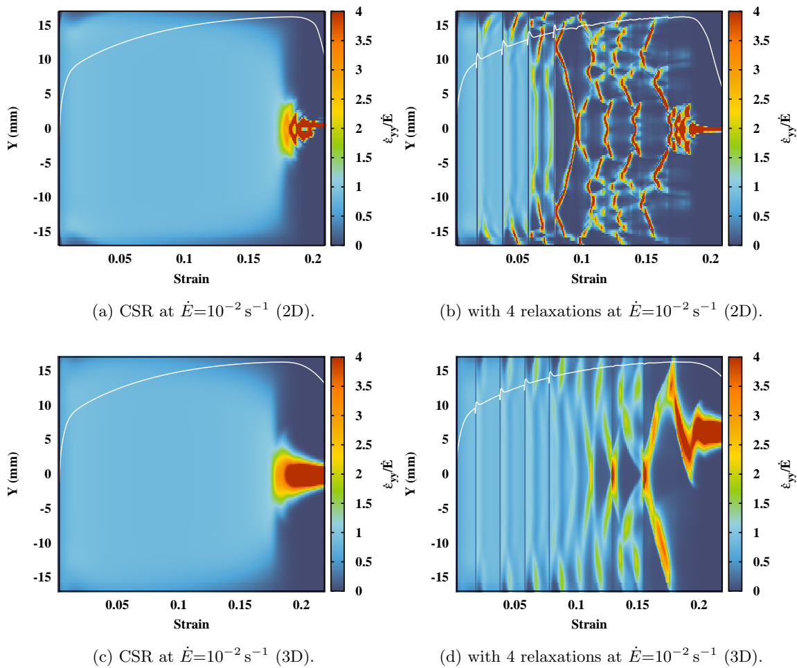
Figure 8: Comparison between numerical spatio-temporal patterns involving 4 relaxations and without relaxation at \dot{E}=10^{-2} \text{ s}^{-1} . The simulations are performed on 2D (a,b) and 3D (c,d) meshes.
