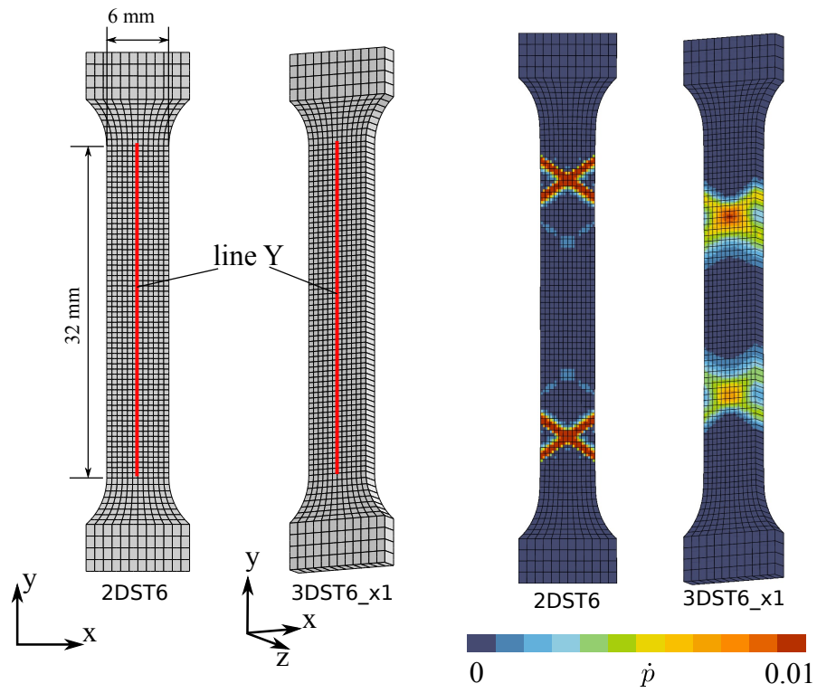
Figure 7: 2D and 3D meshes used for simulations and localization band after the 4th restraining at \dot{E} = 10^{-2} \text{ s}^{-1} .
