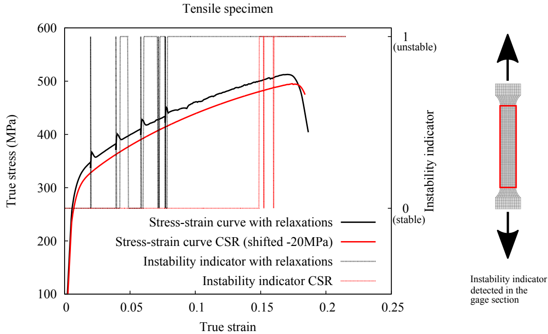
Figure 12: Numerical instability analysis based on a full tensile specimen for both of CSR and relaxation conditions ( \dot{E} = 10^{-2} \text{ s}^{-1} ). The instability indicator is detected in the gauge section.
