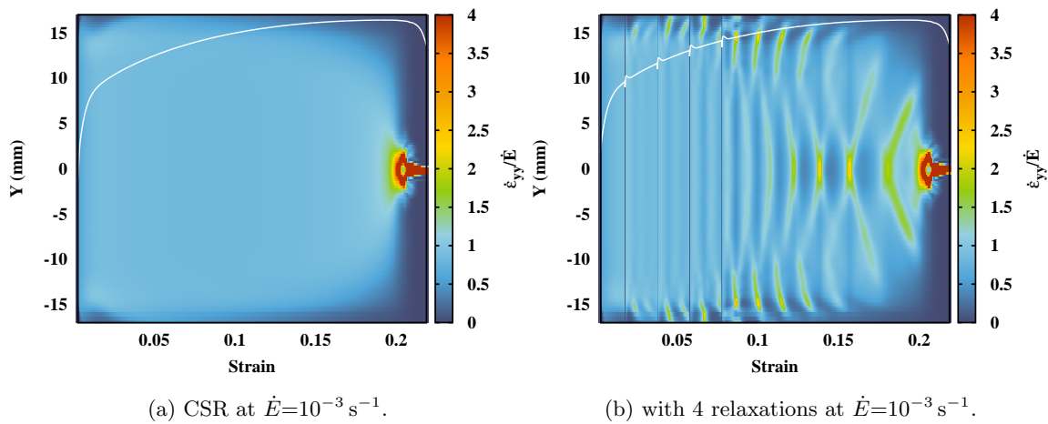
Figure 9: Comparison between numerical spatio-temporal patterns involving 4 relaxations and without relaxation at 10^{-3} \text{ s}^{-1} . The simulations are performed on 2D mesh (2DST6).
