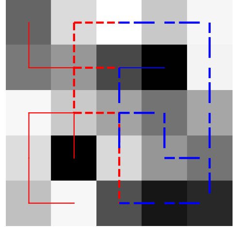
Fig. 2. \mathcal{MST}(\mathbf{I}_0) in red and \mathcal{MST}(I_1) in blue. E_{\mathbf{I}_0} and E_{I_1} in bold and dashed, edges linking common pixels and candidate to form cycles on the union of the two MST.
