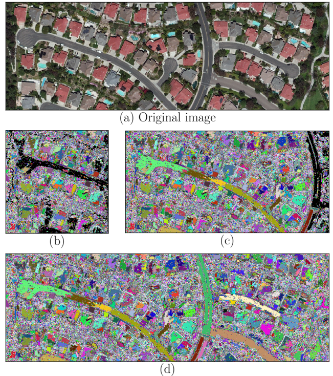
Fig. 5. (b) and (c) Lambda-flat zones ( \lambda = 5 ) computed on streaming by the proposed algorithm on MST. Pixels in black are those that are waiting to a definite label in the streaming process. (d) Final result on the complete image.
