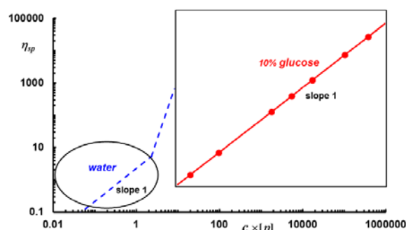
Figure 8: Regions where the linear dependence \eta_{sp} \sim c \times [\eta] was observed for HPC in different solvents at 25 °C
