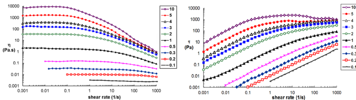
Figure 3: Flow curves for HPC sample with M = 1.15 \times 10^6 \text{ g/mol} and different concentrations (g/dL) in water at 25^\circ \text{C}
