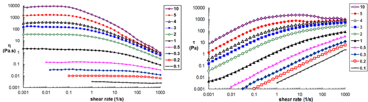
Figure 3: Flow curves for HPC sample with M = 1.15 \times 10^6 \text{ g/mol} and different concentrations (g/dL) in water at 25 \text{ }^\circ\text{C}
