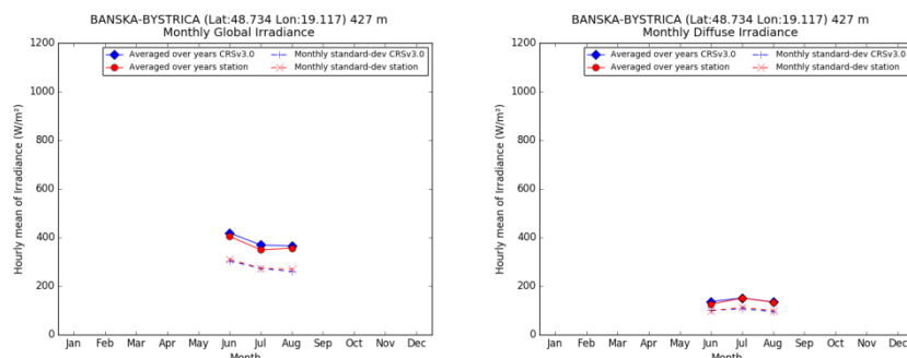
Figure 4. Monthly means of Hourly Mean of Irradiance measurements at station (red dots) and CRSv3.0 (blue diamonds), and monthly standard-deviation of measurements (red crosses) and CRSv3.0 (blue crosses)
