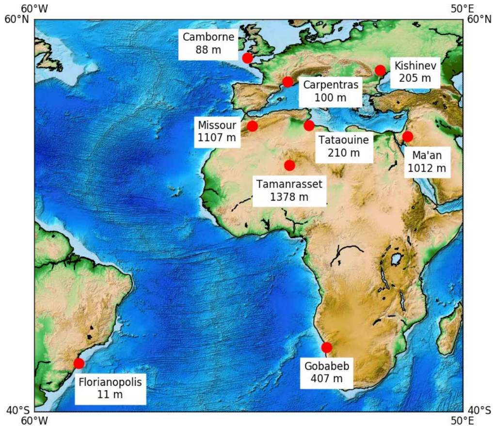
Figure 2.2. Map showing part of the stations. Symbols code the initial summarization: circle for 1 min, and downward triangle for 1 h. Colors code the type of data at each site: red for ( G , B , D ), yellow for ( G , B ), magenta for ( G , D ) and cyan for G .
