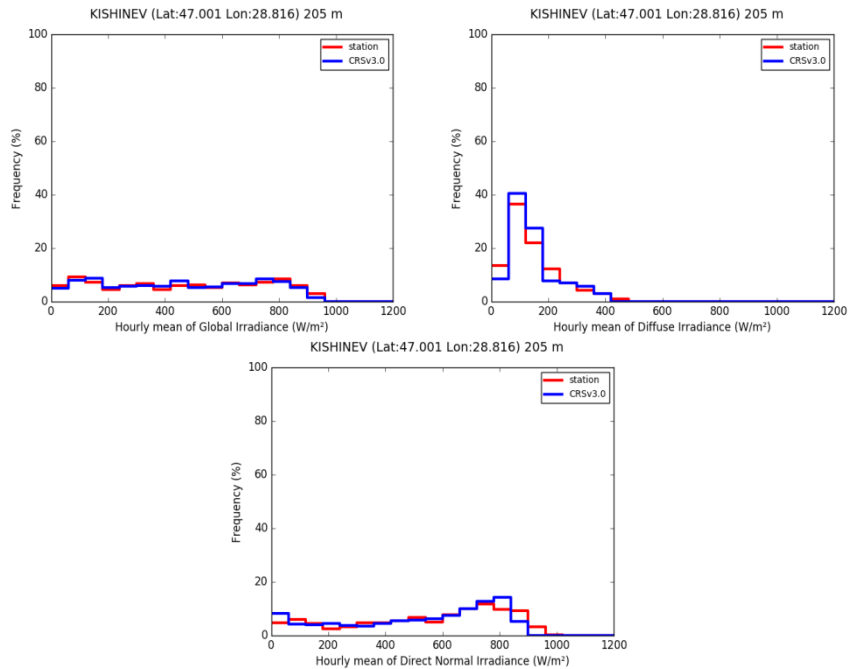
Figure 3. Frequency distributions of the measurements station (red line) and CRSv3.0 (blue line) for Hourly Mean of Irradiance
