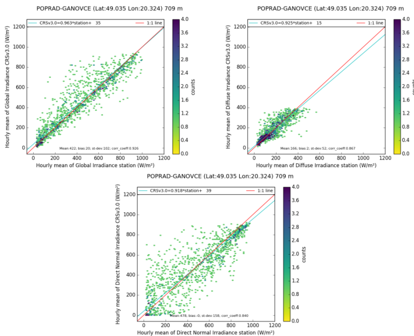
Figure 1. 2-D histogram between ground measurements (station) and the CRSv3.0 product for Hourly Mean of Irradiance
