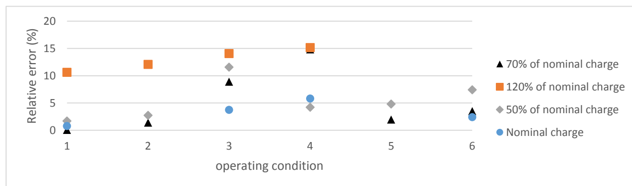
Figure 8: Relative error on heating capacity for different operating conditions and charge fault intensities
