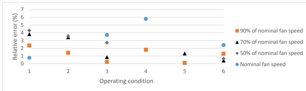
Figure 7: Relative error on heating capacity for different operating conditions and evaporator fault intensities
