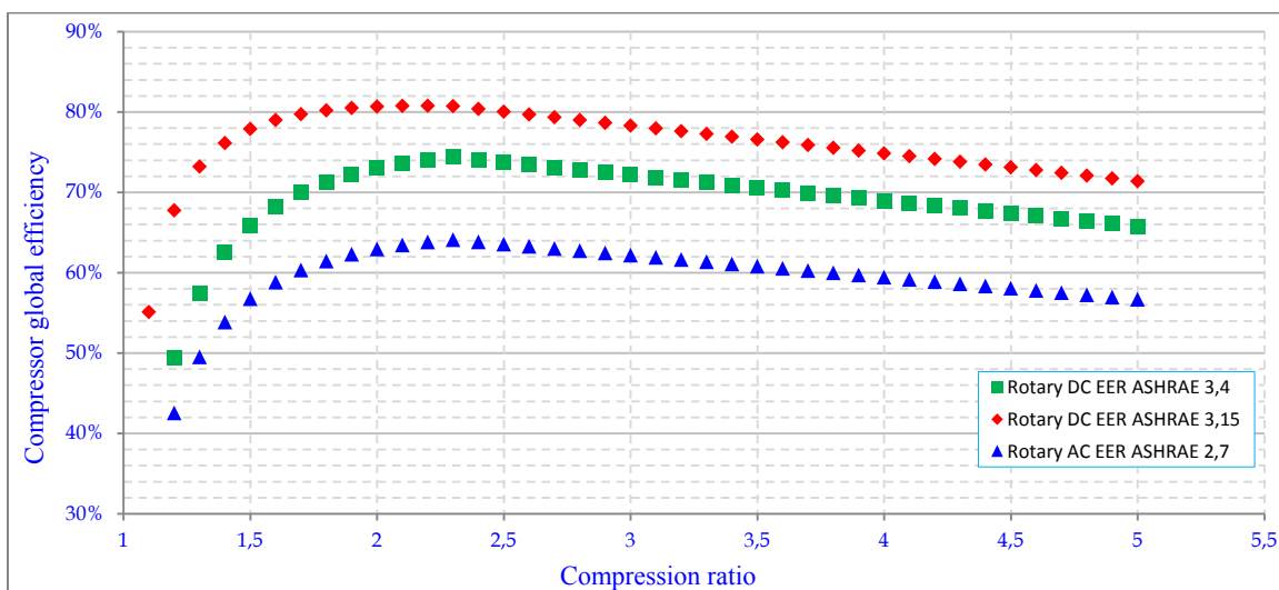
Figure 1: Compressor efficiency curve as a function of the compression ratio for the different compressor options
