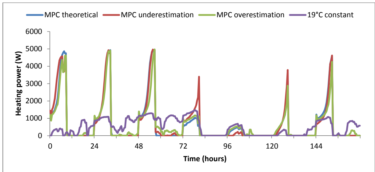
Figure 11: Heating power calculated for case study 2
