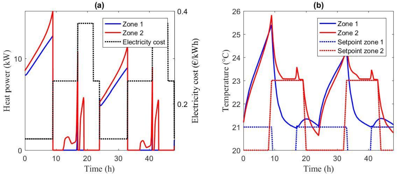
Fig. 4. Decomposition-coordination method results : (a) optimal heating power profiles, (b) resulting temperature profiles
