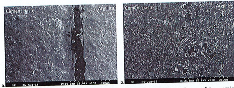
Fig. 2. Very different cement/argillite interfaces are obtained after 2 months depending (a) on whether a hardened cement disk was put into contact with the argillite disk or (b) the cement was directly poured onto the argillite (SEM images in SEB-SE mode, i stands for interface).
