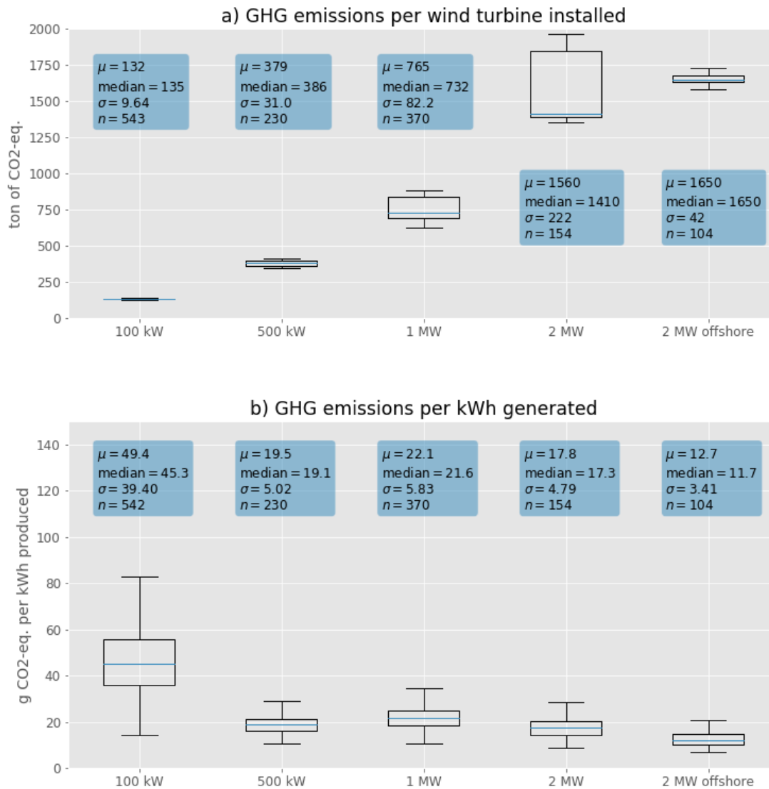
312 Figure 5: Statistical distribution of wind turbines GHG emissions per power category expressed as: a) emissions per life cycle and 313 b) emissions per kWh produced. The blue horizontal line is the median value. Vertical rectangles represent 50% of the distribution. 314 Vertical black intervals represent 90% of the distribution. Outlying values are computed but not displayed.
