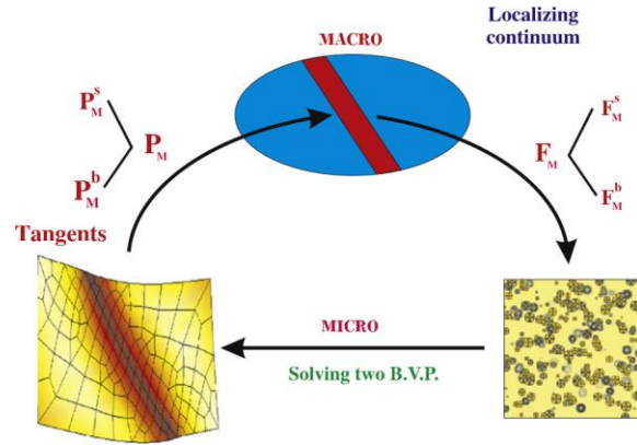
Fig. 14 Continuous-discontinuous homogenization scheme. A deformation gradient for the unloading material ( F_M^s ) and one for the localization band ( F_M^b ) is transferred from the macroscopic model to two different microscopic models. The microscopic models produce the homogenized responses represented here by two tangent moduli and two first Piola-Kirchhoff stress tensors for the respective zones. Reprinted from Geers et al (2010), with permission from Elsevier.
