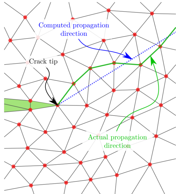
Fig. 7 Prescribed crack path (dashed blue line) and the actual crack path (solid green line) after cohesive elements insertion.
