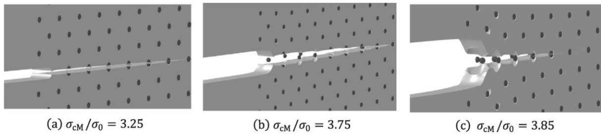
Fig. 8 FE simulation of a ferritic steel microstructure using CZMs at particles/matrix interfaces, and along a predefined crack propagation path through particles and matrix at the midsection of the specimen. The ratio \sigma_{cM}/\sigma_0 is the ratio between matrix cohesive strength and matrix yield stress. Reprinted from Giang et al (2017), with permission from Elsevier.
