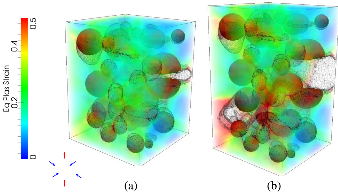
Fig. 18 Micromechanical simulation of a metal matrix composite microstructure showing void nucleation by particles debonding and fragmentation, growth and coalescence modeled using remeshing at an applied tensile strain of: (a) 25 % and (b) 50%. Particles are shown in red and the color code in the matrix is associated to the equivalent plastic strain. Reprinted from Shakoor et al (2017a), with permission from Elsevier.
