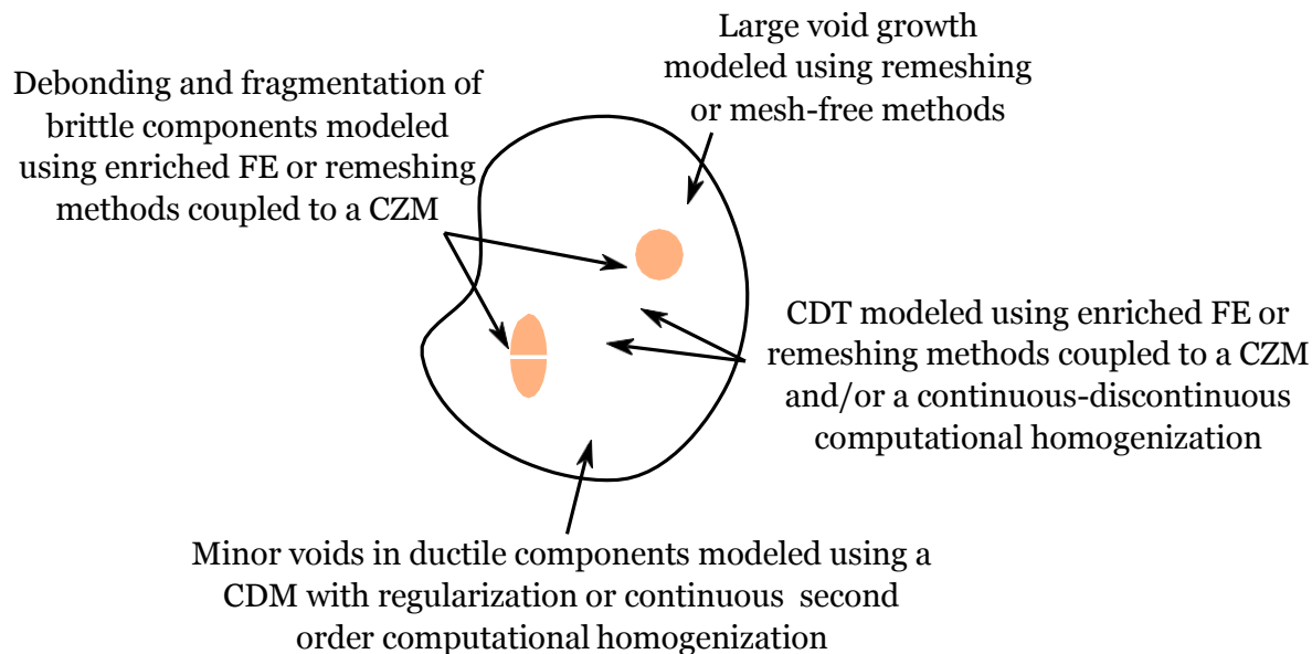
Fig. 19 Main approaches retained in the present review for numerical modeling of ductile fracture at the microscale.
