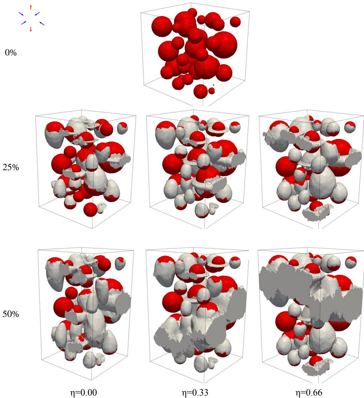
Fig. 9 Micromechanical simulations of a metal matrix composite microstructure showing remeshing based modeling of void nucleation by particle debonding and fragmentation followed by void growth and coalescence. Voids are shown in light gray, particles in red, and \eta refers to the stress triaxiality ratio. Reprinted from Shakoor et al (2017a), with permission from Elsevier.
