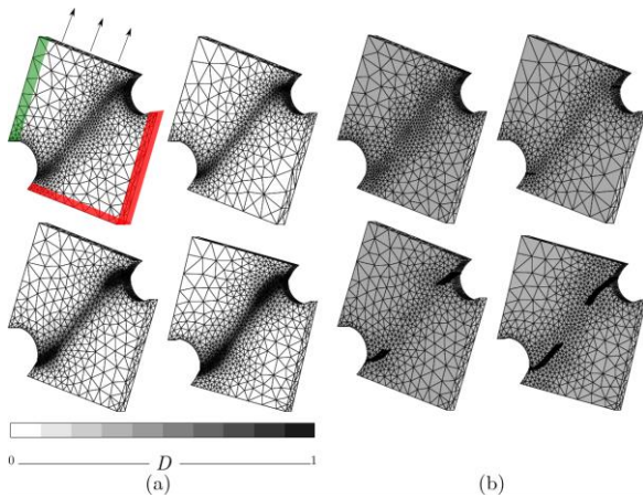
Fig. 16 Double notched 3D specimen test case result at four load increments. Arrows point out the loading direction. Red faces are fixed. Green face is sliding along the loading direction. (a) View of the continuous damage field D . (b) View of the two cracks. Reprinted from Feld-Payet (2010).
