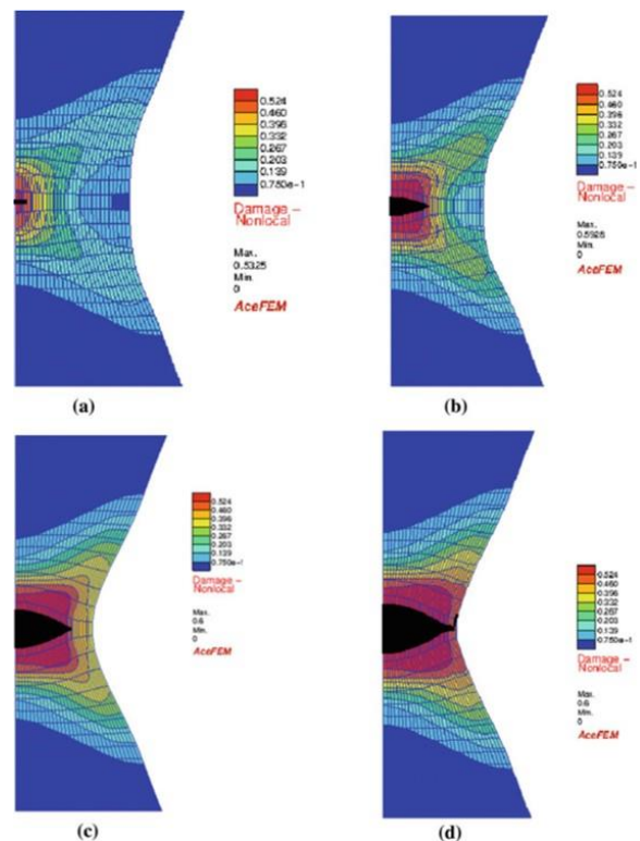
Fig. 13 Damage and crack evolution in a plane strain specimen from crack initiation up to final failure. Reprinted from Seabra et al (2013), with permission of Springer.
