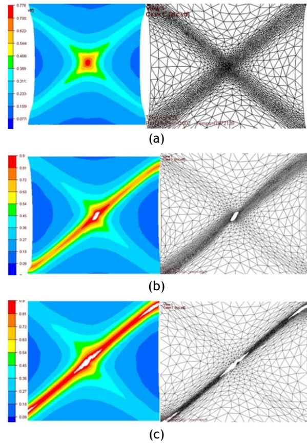
Fig. 15 Cross sections of a 3D tension test simulation using ductile fracture modeling by element erosion and anisotropic mesh adaption at an engineering tensile strain of: (a) 21.80%, (b) 22.05%, (c) 22.10%. Damage distribution is shown on the left, and the adapted FE mesh on the right. Reprinted from El khaoulani and Bouchard (2013), with permission from Elsevier.
