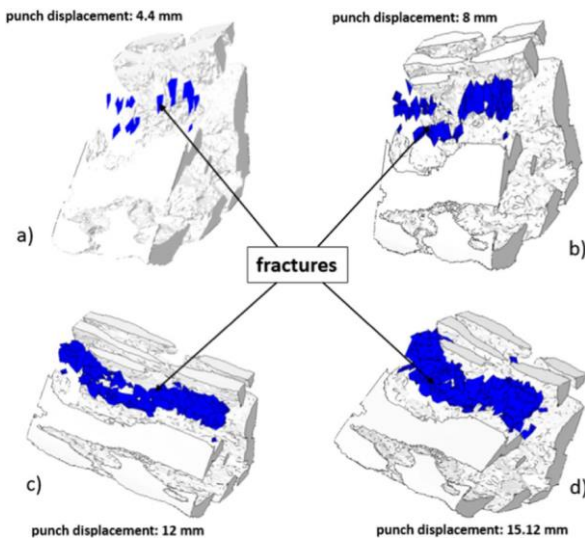
Fig. 3 Micromechanical simulation of a 3D dual phase steel microstructure showing in white the martensite phase, and in blue eroded elements from the ductile ferrite phase. The reader is referred to Perzyński et al (2017) for indications on the relation between punch displacement and boundary conditions at the microscale. Reprinted from Perzyński et al (2017), with permission from Elsevier.
