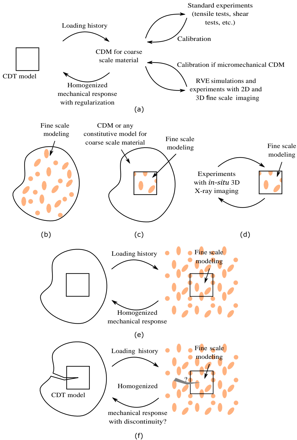
Fig. 11 Summary of continuous approaches: (a) Empirical, phenomenological or micromechanical CDMs; (b) DNS using fine scale models; (c) DNS using fine scale models only in a region of interest, using a CDM elsewhere; (d) DNS using fine scale models only in region of interest and measured boundary conditions based on in situ 3D X-ray data; (e) Computational homogenization using periodic boundary conditions; (f) Computational homogenization with CDT modeling.
