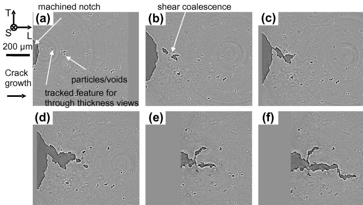
Fig. 1 Cross section from 3D X-ray images of the microstructure of a thick notched specimen under tensile loading at different crack mouth opening displacements: (a) 0 mm, (b) 1.625 mm, (c) 1.875 mm, (d) 2.0625 mm, (e) 2.3125 mm, (f) 2.375 mm. The material, an aluminum alloy with less than 1% initial particles/voids volume fraction, fails by the initiation and propagation of a macroscopic crack in a zig-zag pattern due to the influence of the microstructure. Reprinted from Morgeneyer et al (2011), with permission from Elsevier.
