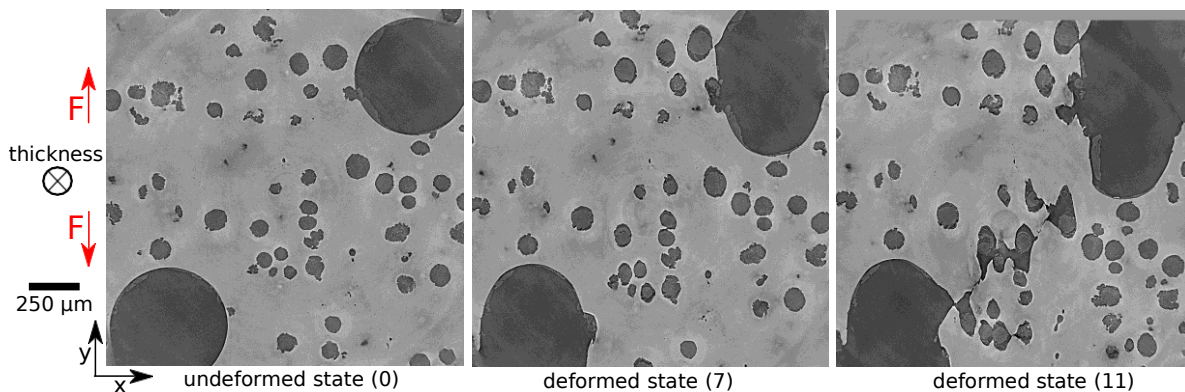
Fig. 2 Cross section from 3D X-ray images of the microstructure of a flat specimen with two machined holes at 45° under tensile loading. The material, nodular cast iron, fails by debonding and fragmentation of the nodules, and then void growth, coalescence and sheeting in the shear band between the two machined holes. Reprinted from Shakoor et al (2017c), with permission from Elsevier.
