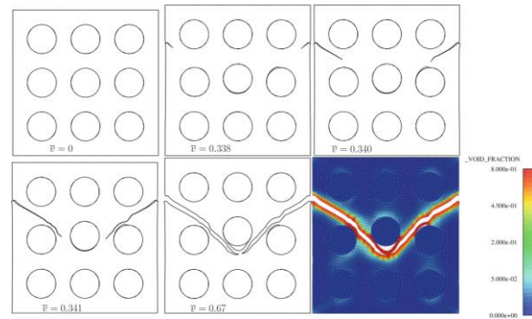
Fig. 17 FE simulation of a 2D inclusions array using remeshing based cracks initiation and propagation. Results are shown at various applied displacement v . Reprinted from Areias et al (2011), with permission of Springer.
