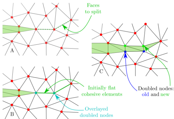
Fig. 6 Schematic representation of the insertion of a cohesive element: A. The green dashed line shows the faces that will be split. B. The cyan dots correspond to the nodes that have been doubled and therefore there are indeed two nodes at the same location. The green line corresponds to a initially flat cohesive element. C. After loading the new inserted cohesive elements open.
