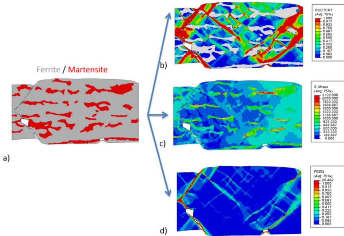
Fig. 4 Micromechanical simulation of a 2D dual phase steel microstructure showing the ductile fracture of the ferrite phase modeled using element deletion and the brittle failure of the martensite phase modeled using X-FEM. (a) Microstructure with ferrite in gray and martensite in red. (b) Damage variable in ferrite phase. (c) Von Mises stress field. (d) Equivalent plastic strain field. Reprinted from Perzyński et al (2017), with permission from Elsevier.
