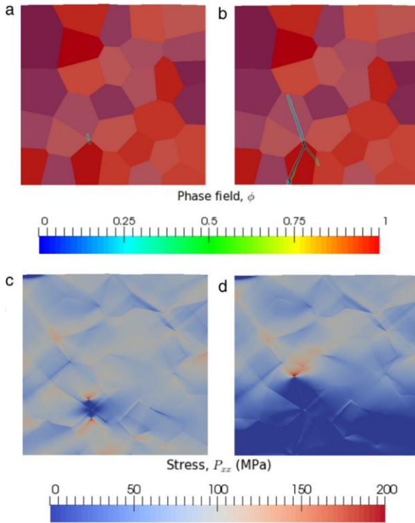
Fig. 12 Evolution of the damage PF variable ( \phi ) and stress in a polycrystalline patch loaded in the horizontal direction at an applied tensile strain of: (a, c) 1.16%, (b, d) 1.21%. Reproduced from Shantraj et al (2016), with permission from Elsevier.
