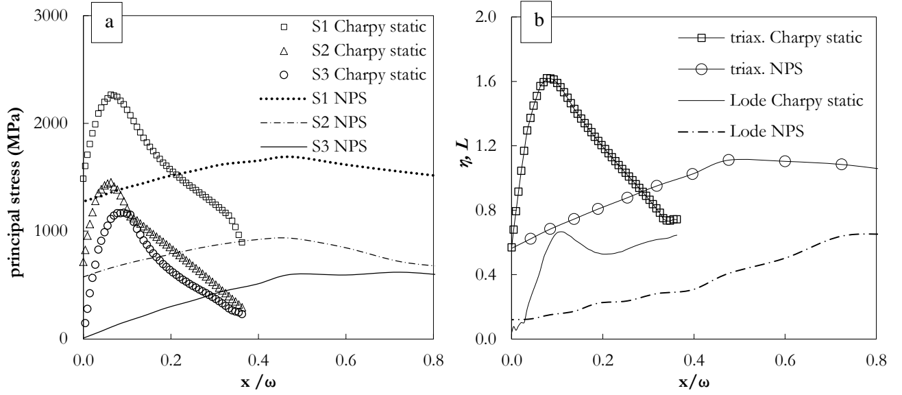
Fig. 13: Comparison of estimated evolutions of (a) principal stresses ahead of the notch tip and (b) estimated stress triaxiality and Lode parameter along the ligament between (static) Charpy and NPS specimens.
