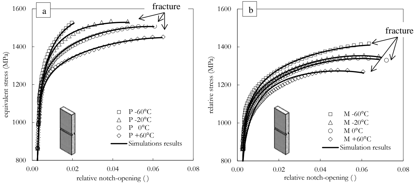
Fig. 10: Results of tensile tests at different temperatures on NPS specimens of (a) microstructure P (b) microstructure M.
