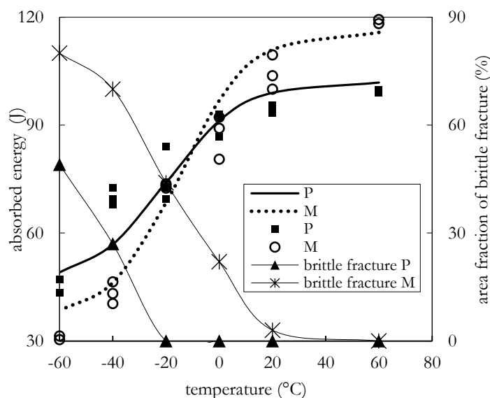
Fig. 6: Charpy impact properties of the tested steels and area fraction of brittle fracture.
