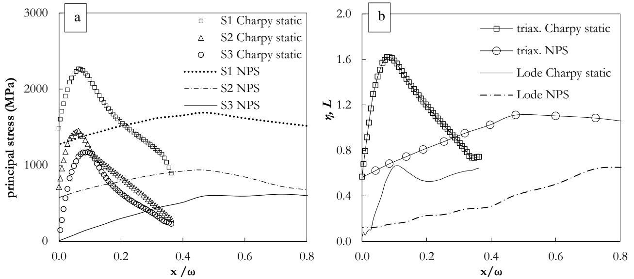
Fig. 13: Comparison of estimated evolutions of (a) principal stresses ahead of the notch tip and (b) estimated stress triaxiality and Lode parameter along the ligament between (static) Charpy and NPS specimens.
