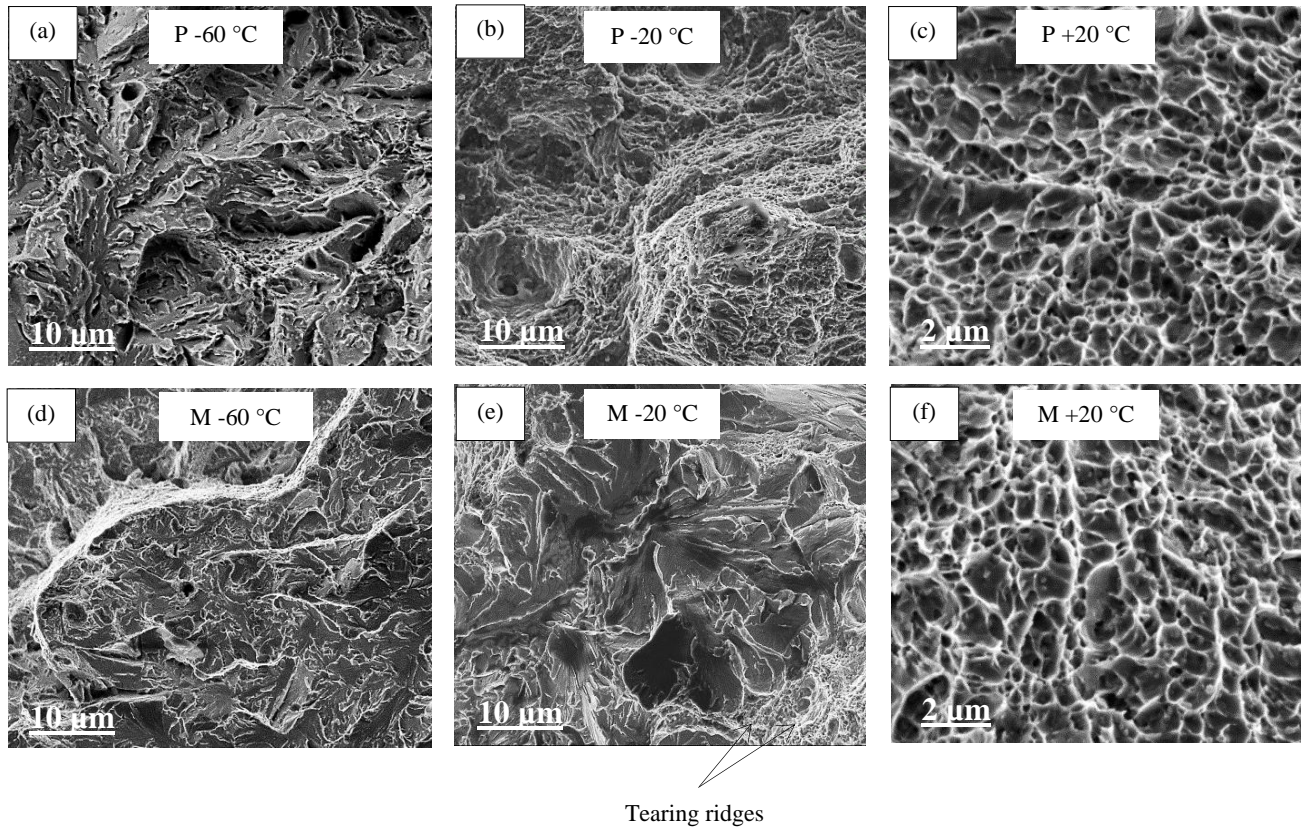
Fig. 7: Fracture surfaces of (a,b,c) P and (d,e,f) M Charpy specimens tested at -60°C, -20°C and at room temperature.
