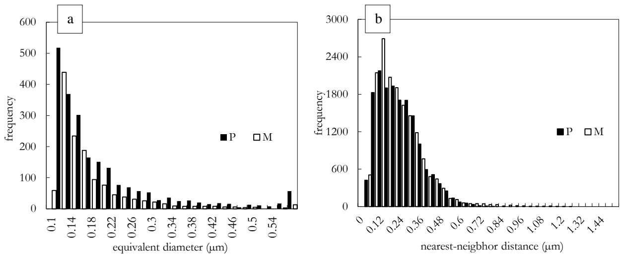
Fig. 3: Results of statistical analysis on M_3C carbides, (a) carbide size distribution, (b) distribution of nearest-neighbor distances between carbides for P and M specimens, respectively.
