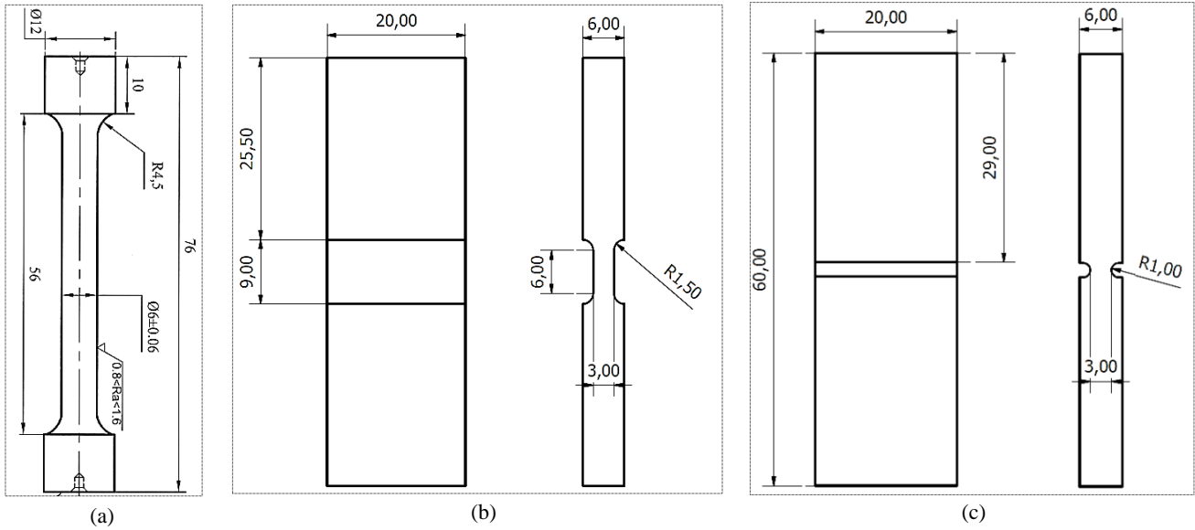
Fig. 1: Dimensions (in mm) of (a) SC. (b) SPS and (c) NPS specimens. All dimensions in mm.
