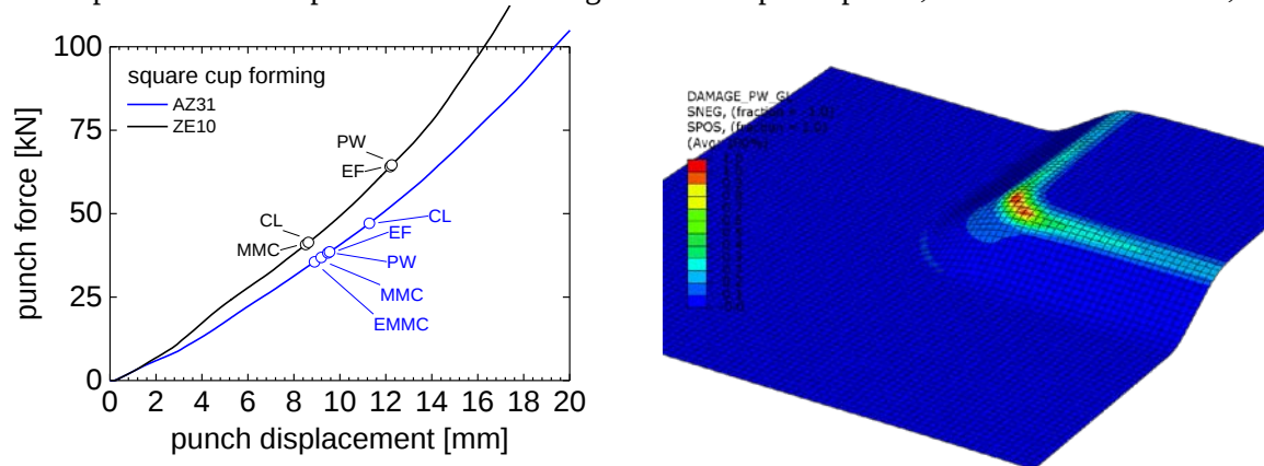
Figure 3. Forming of a square box: (a) predicted failure points for different criteria; (b) corner failure of AZ31 predicted by the plastic work criterion.
