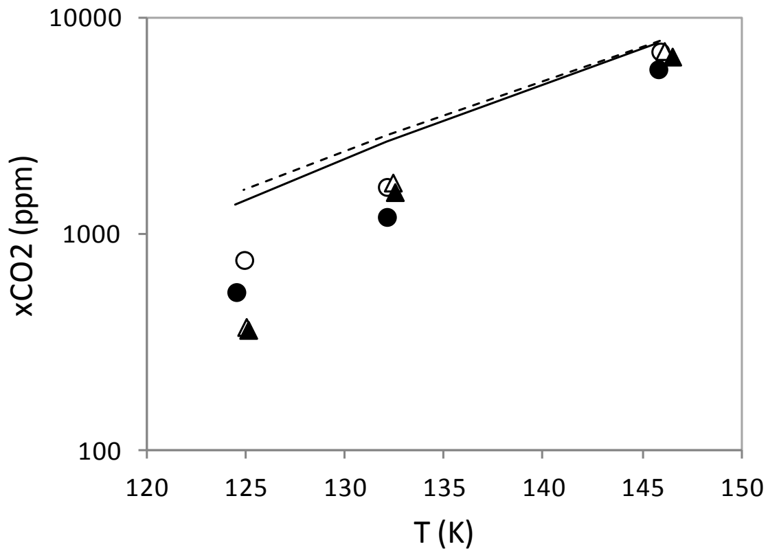
Figure 4. CO 2 solubility in liquid phase ( x_{CO_2} ) at SLVE conditions from experimental values obtained in this work for the N 2 -CH 4 -CO 2 system (○ series 1, ● series 2), and the N 2 -O 2 -CH 4 -CO 2 system (△ series 3, ▲ series 4). Results from the model are almost superposed for the ternary and the quaternary system and then they are represented for the ternary system only (--- first series, — second series), for the sake of clarity.
