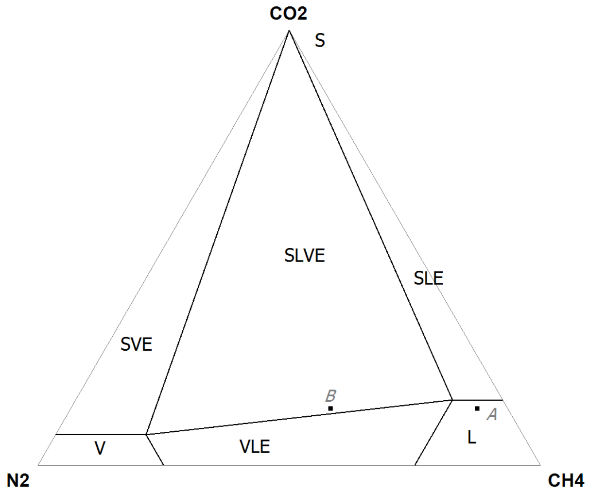
Figure 1. Qualitative phase diagram of the \text{N}_2\text{-CH}_4\text{-CO}_2 system at biomethane liquefaction conditions. S is for solid, L for liquid, and V for vapor phase.
