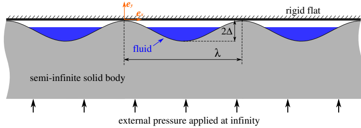
Figure 2: A sketch of the problem under study.
