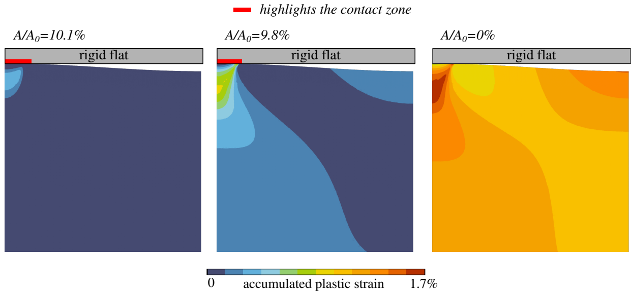
Figure 12: Accumulated plastic strain near the contact interface is shown at three different external loads for the incompressible fluid and for V_f/V_{g0} = 0.9 and \Delta/\lambda = 0.01 , from left to right: (1) the step corresponding to activation of the fluid; (2) the plastic zone appears in the valley between the asperities; (3) opening of the trap (contact area is zero; as seen from the plastic field, at this moment the entire solid is plastified).
