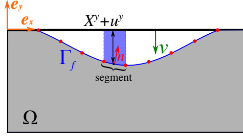
Figure B.16: Trapped fluid element, consisting of all segments of the surface boundary \Gamma_f (shaded in blue is the part of the trapped fluid volume, which corresponds to the highlighted segment).
