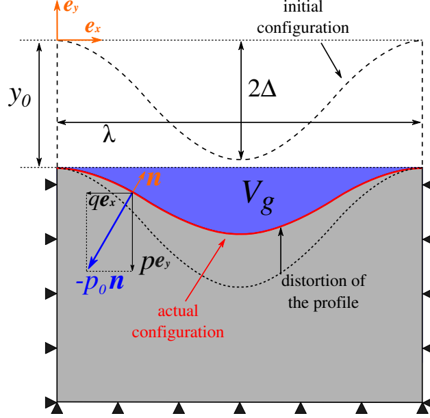
Figure A.15: Distortion of a periodic wavy surface under a uniform hydrostatic pressure.
