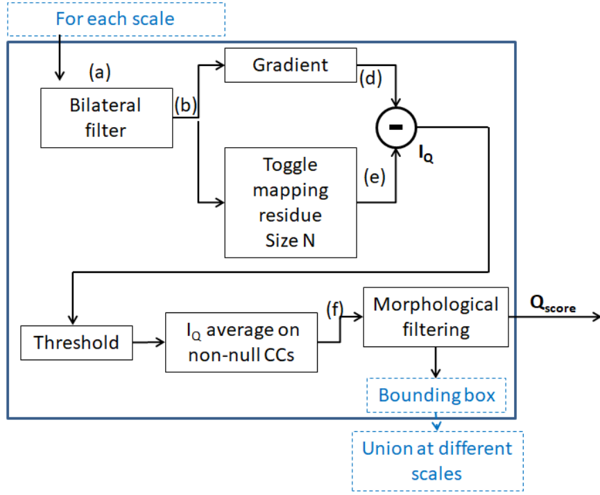
Fig. 2. Algorithm flowchart.
