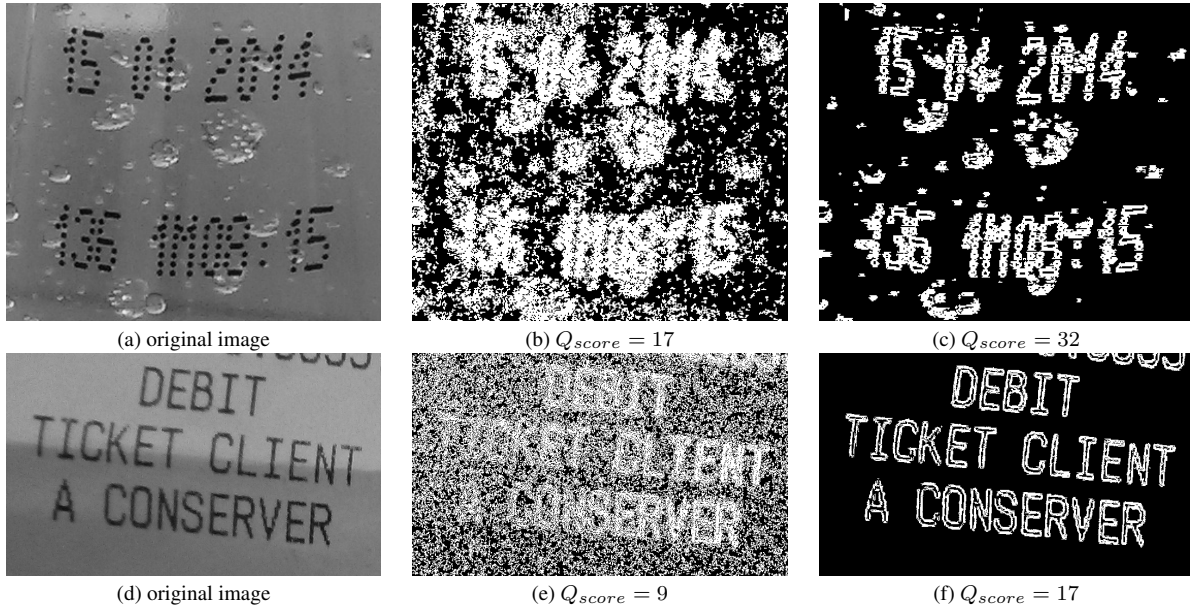
Fig. 3. Filter influence in I_Q computation. Left column: original image. Middle column: Thresholded I_Q computed from original image. Right column: Thresholded I_Q from bilateral filtered image.
