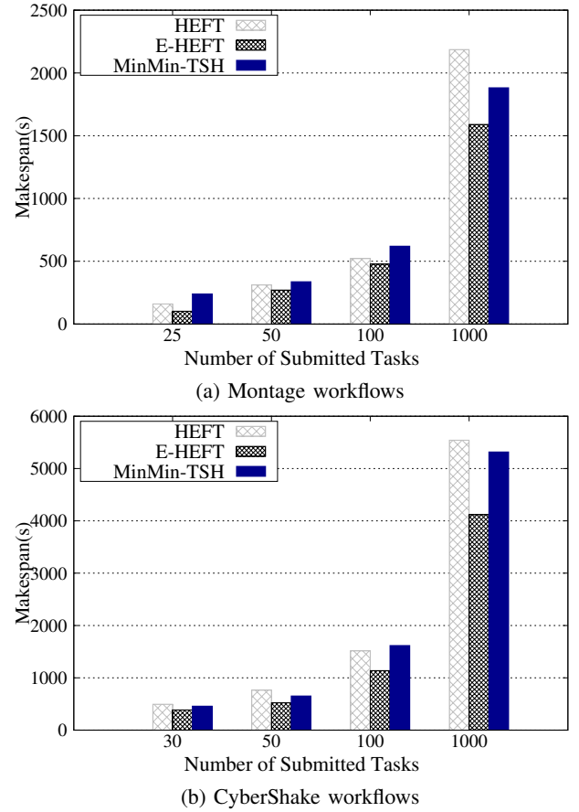
Fig. 6: Average makespane of the three algorithms based on Montage and Cybershake workflows.
