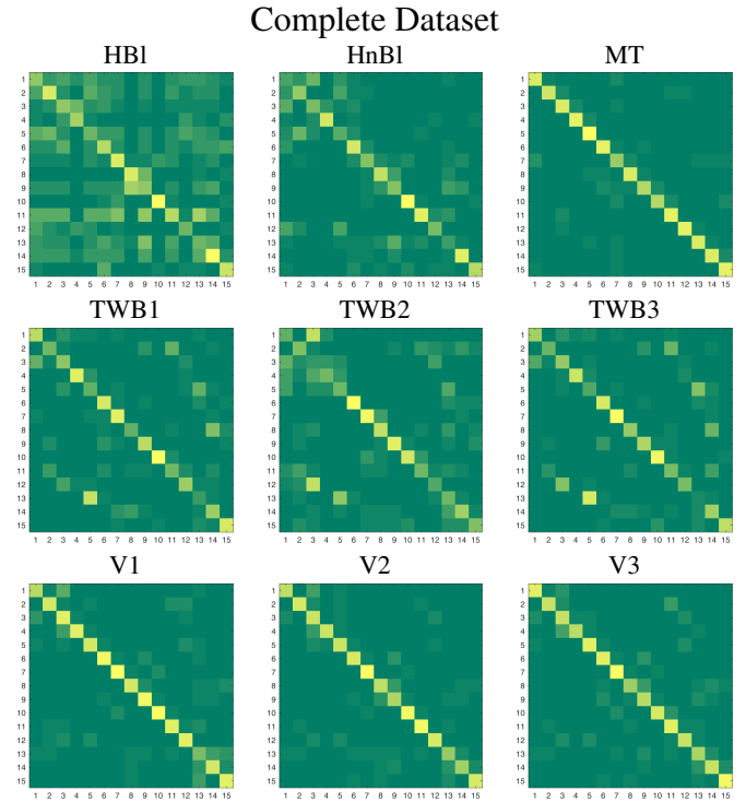
Figure 8: Confusion matrices over the complete dataset.
