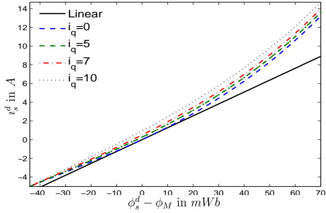
(a) i_s^d as a function of \phi_s^d for may values of i_s^q (in A)
