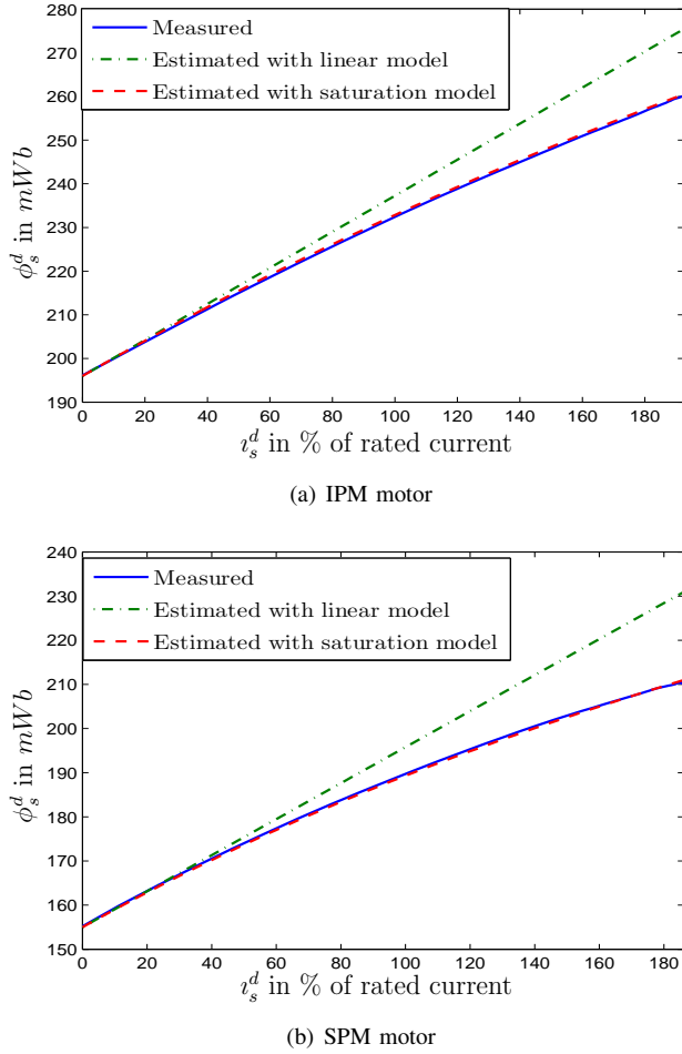
Fig. 4. Experimental and fitted flux-current relations.
