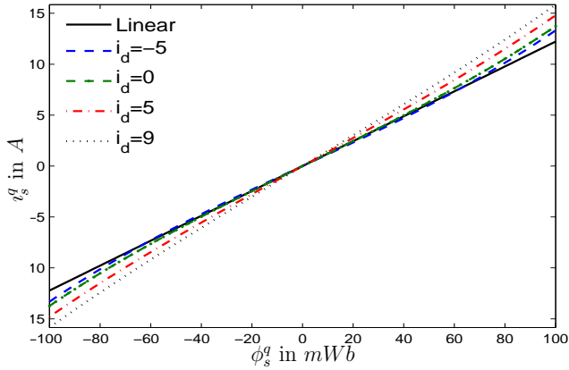
(b) i_s^q as a function of \phi_s^q for may values of i_s^d (in A)
