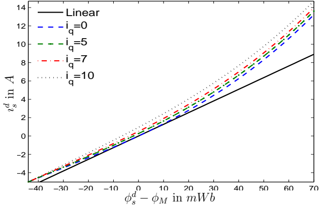
(a) \lambda_s^d as a function of \phi_s^d for may values of i_s^q (in A)
