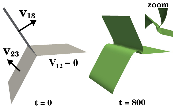
Figure 8: Three grain junction with initial angles of 120 degrees with imposed constant velocities and results of 3D simulations of junction motion by the LS method (similar to the 2D case shown in Fig. 6).
