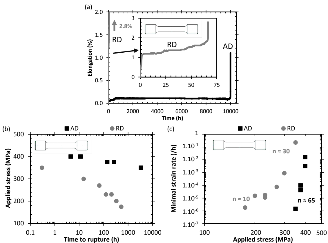
Figure 3. Creep tests results at 650^{\circ}\text{C} on smooth specimens. (a) Creep curves under 270 MPa; (b) Monkman-Grant plot and (c) Norton-like strain rate vs. stress plot.
