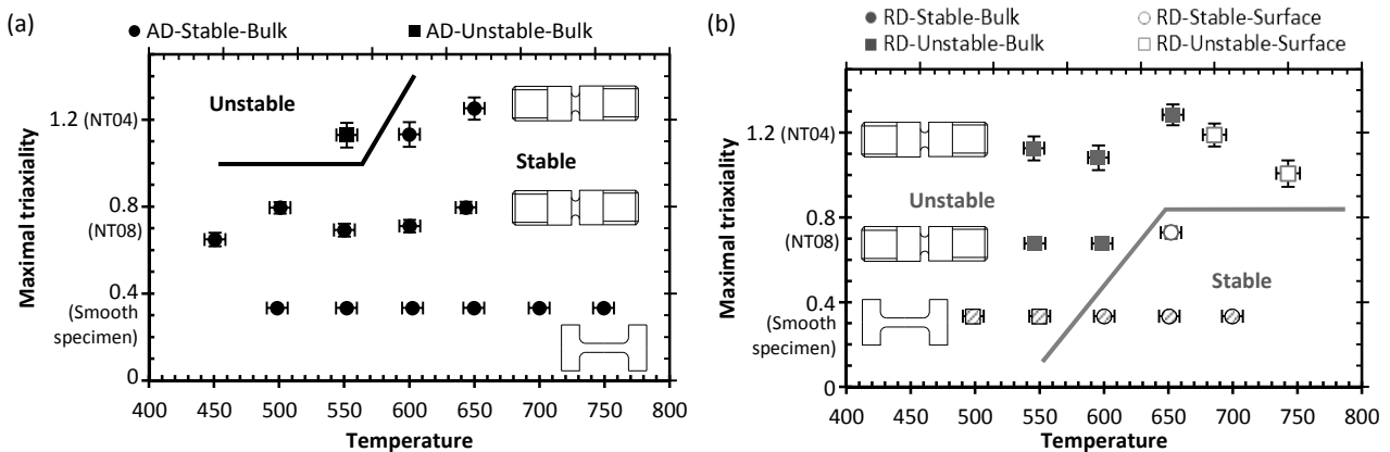
Figure 9. Crack initiation location (from close to the specimen side surface or from the bulk) and global fracture stability during tensile tests, as a function of initial maximal stress triaxiality and test temperature along (a) AD and (b) RD (for which crack initiation location could not be determined in smooth specimens). Lines delineate the boundary between regions of unstable and stable fracture behavior, respectively.
