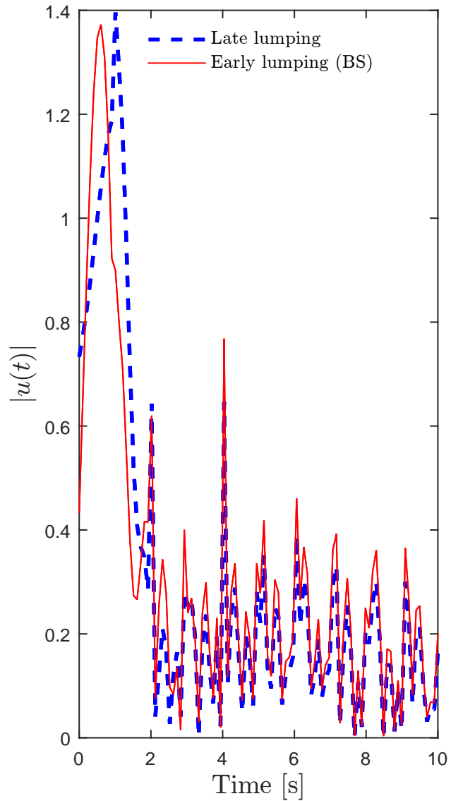
Control effort
