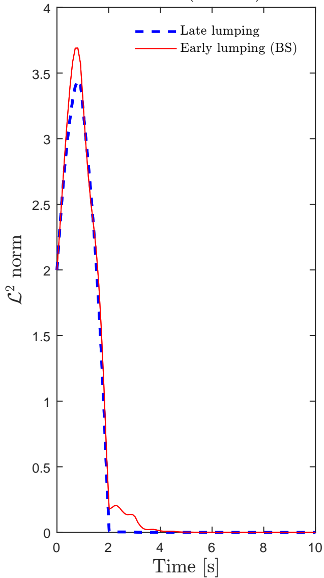
\mathcal{L}^2 -norm (1 mode)
