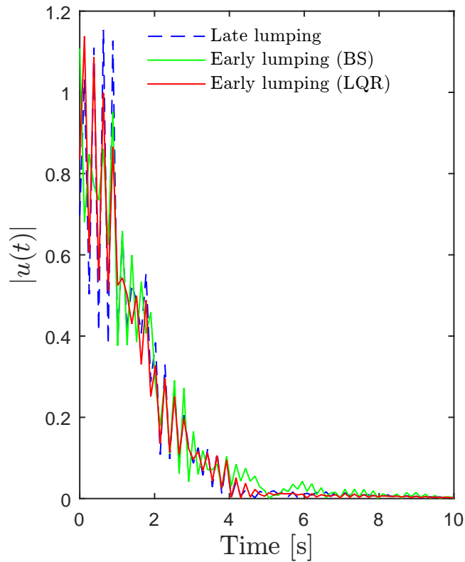
Control effort
