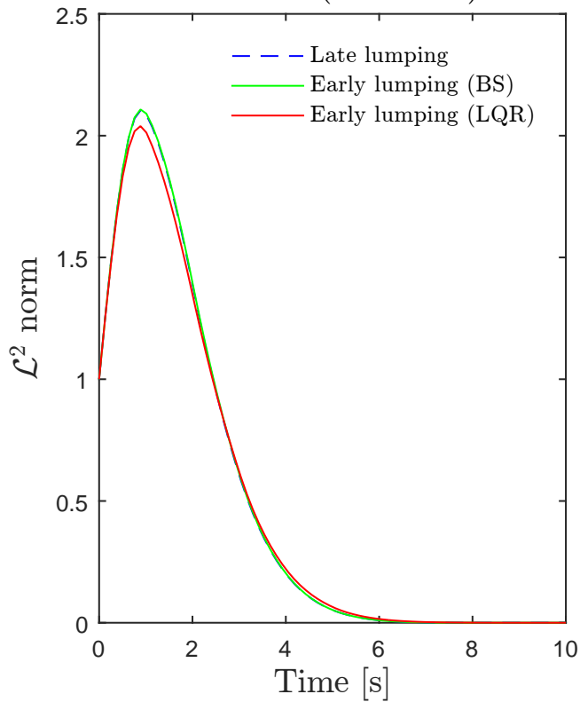
\mathcal{L}^2 -norm (40 modes)
